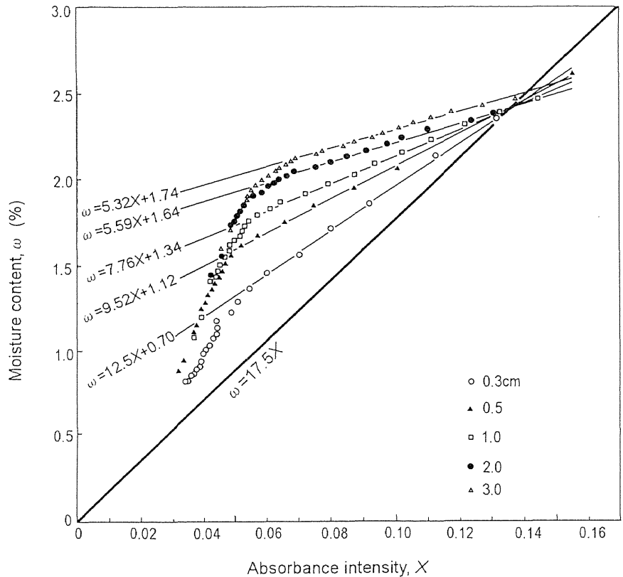
Fig. 1. The relationships between absorbance ( X -value) and moisture content ( w ) for a variety of disc thicknesses.
