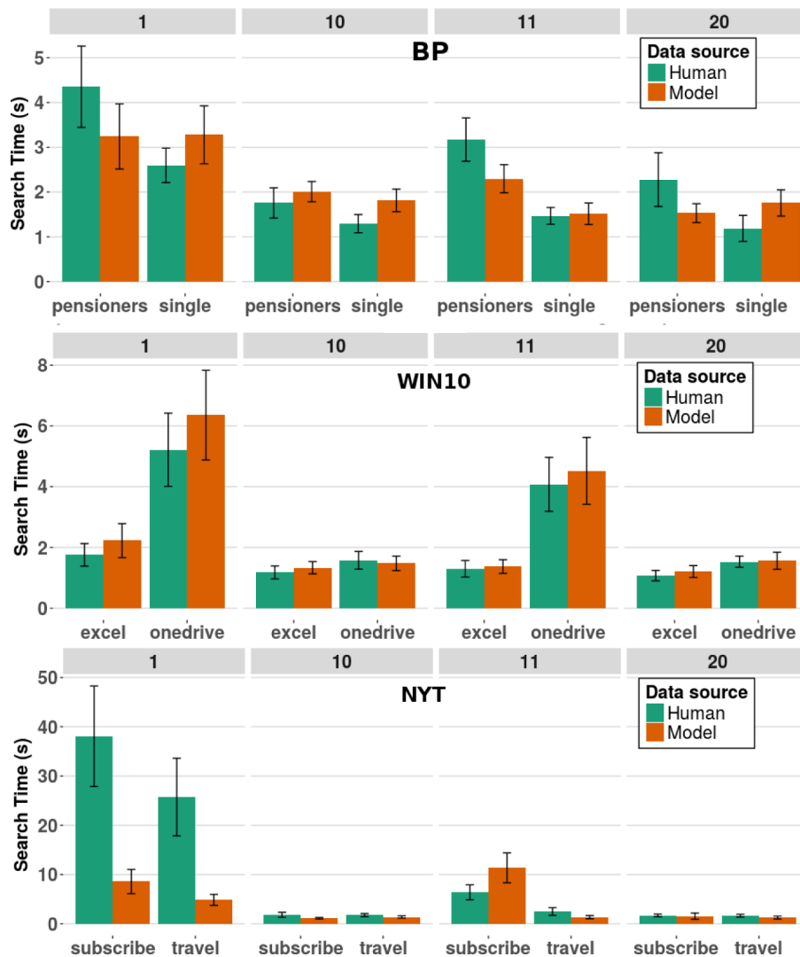
Fig. 9. Human and model search times in the initial and final phases for two elements in the three layouts. In the beginning of layout learning (1 min), more salient targets (e.g., 'excel'), are faster to find than non-salient targets ('onedrive'). Right before the layout change (10), all elements can be found quickly. After layout change (11), moved elements are slower to be found ('pensioners', 'onedrive' and 'subscribe'). After relearning (20), the search for everything is quick again. Error bars are standard errors with N = 20 .
