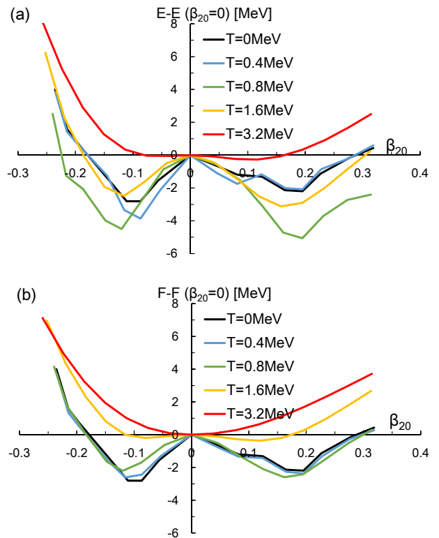
FIG. 7. Potential energy surface, calculated with the constrained FT-HFB method, as a function of the quadrupole deformation, for ^{184}\text{Hg} . The panel (a) is the total energy E , while the panel (b) is the free energy F . See text for details.
