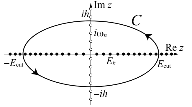
FIG. 1. Schematic illustration of the contour C and poles of the Green's function G(z) (closed circles) and of the Fermi-Dirac function f_T(z) (open circles) in the complex plane.
