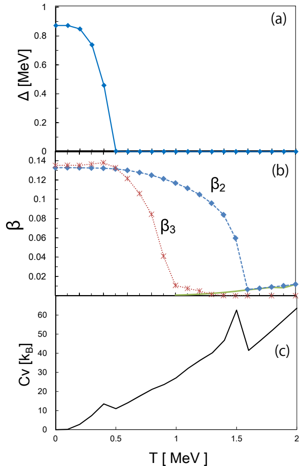
FIG. 5. (a) Calculated neutron average pairing gap, (b) quadrupole and octupole deformation parameters, and (c) specific heat as functions of temperature for ^{146}\text{Ba} . In the panel (b), the quadrupole deformation of the dripped uniform neutrons is shown by the solid line.
