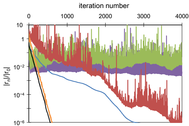
FIG. 3. The convergence behavior of the shifted COCG and shifted COCR methods for solutions of Eq. (28). Three typical points, z(\theta = 0) (COCG/COCR: purple/green) and z(\pi/2) (orange/black), have been taken as examples. The norms of the residual vectors |r_k^\sigma/r_0^\sigma| are shown as functions of the iteration number. This is a case of the FT-HFB calculation for the center of mass of a ^{146}\text{Ba} nucleus ( \mathbf{r}' = \mathbf{r}_c ) with the temperature of k_B T = 200 keV. The mesh and box sizes are the same as those in Sec. III C.
