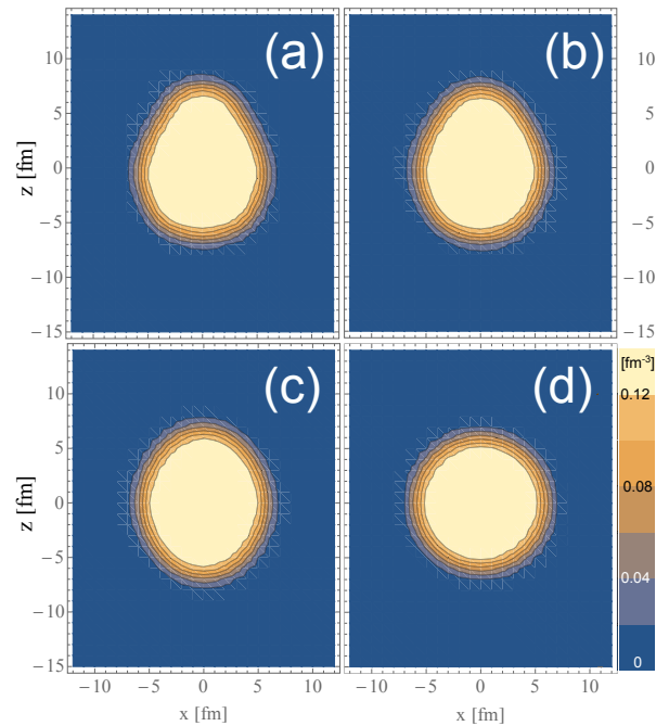
FIG. 6. Nucleon density profiles in the z-x plane for ^{146}\text{Ba} at different temperature; (a) T = 0 , (b) k_B T = 0.8 MeV, (c) k_B T = 1.2 MeV, and (d) k_B T = 1.6 MeV.
