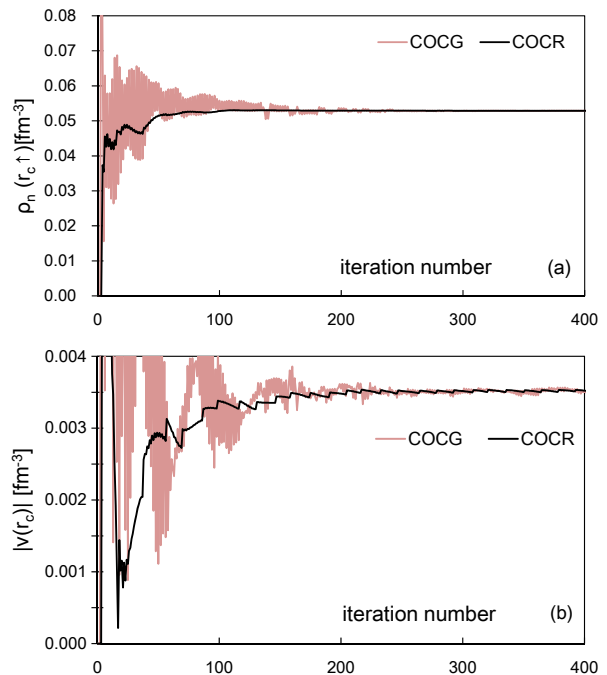
FIG. 4. The convergence behavior of (a) the neutron spin-up density \rho(\mathbf{r}' \uparrow, \mathbf{r}' \uparrow) , and (b) the neutron pair density \nu(\mathbf{r}') = \kappa(\mathbf{r}' \uparrow, \mathbf{r}' \downarrow) at the center of mass of a ^{146}\text{Ba} nucleus ( \mathbf{r}' = \mathbf{r}_c ) with k_B T = 200 keV. The shifted COCG method is shown by red lines and the shifted COCR methods by black lines. See text for details.
