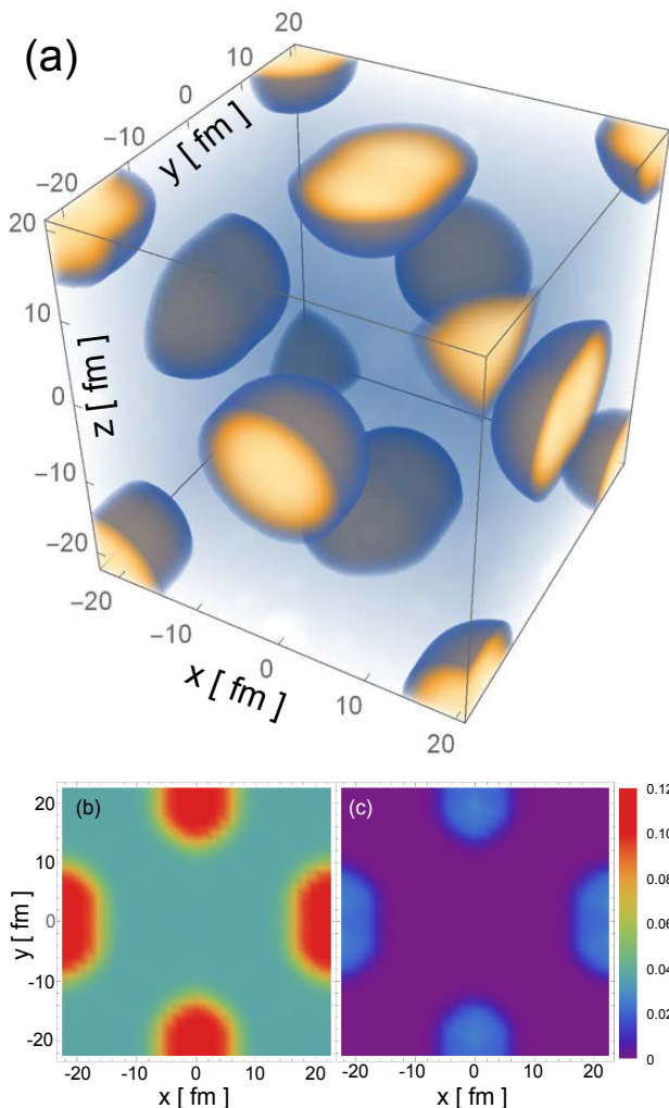
FIG. 8. Nucleonic density distribution in the inner crust of neutron stars at beta equilibrium with the neutron chemical potential \mu_n = 10 MeV and the proton chemical potential \mu_p = -58.5 MeV: (a) 3D plot of baryon density, (b) 2D contour plot of neutron density in the z = 0 plane, and (c) the same as (b) but for protons.
