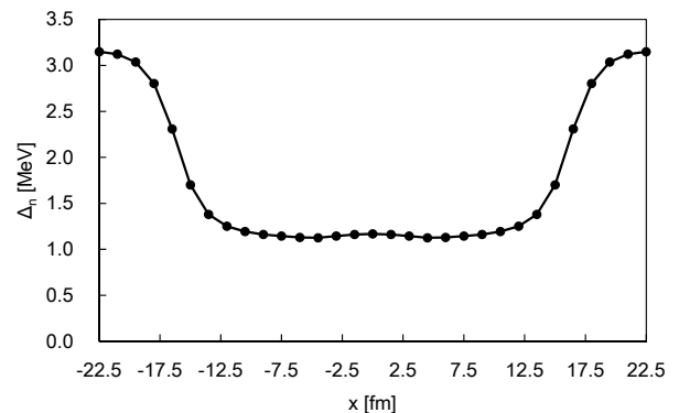
FIG. 9. Calculated neutron gap \Delta_n(\mathbf{r}) on the x axis. The protons are clustered near the both edges.
