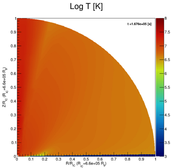
Figure B2. The density (top) and temperature (bottom) structure of small disc simulation.
