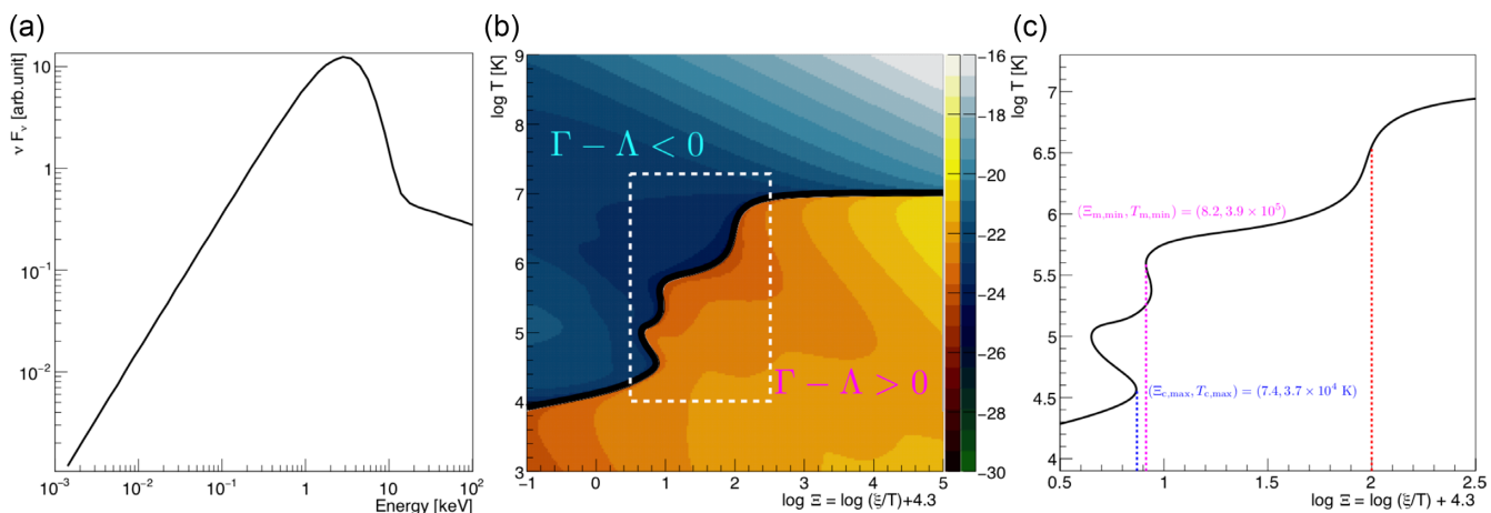
Figure 1. (a) The energy flux of H1743–322 that consists of a disc blackbody plus Comptonized power law (DISKBB+DISKBB*SIMPLE in XSPEC). (b) The heating and cooling function ( \Gamma - \Lambda ). The black curve shows the thermal equilibrium ( \Gamma - \Lambda = 0 ), the right-hand colour bar shows the absolute logarithm value of heating minus cooling function ( \log|\Gamma - \Lambda| ). The Compton temperature of this spectrum is T_{IC} = 1.0 \times 10^7 K. (c) The zooming figure of (b) surrounding by white dashed line. The vertical lines show the instability points. Red vertical lines are \Xi_{h,\min} = 100 .
