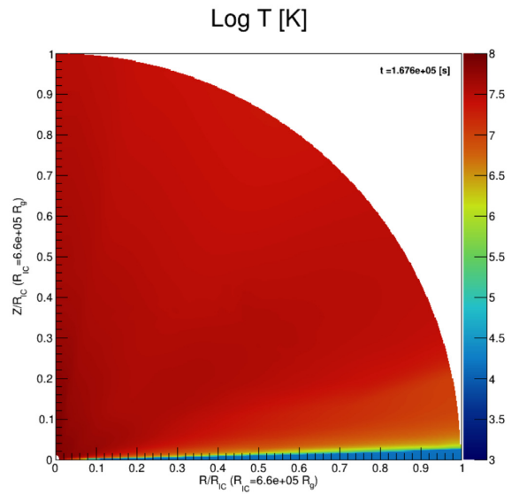
Figure B3. The density (top) and temperature (bottom) structure of hard state.
