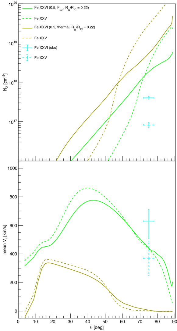
Figure 6. As in Fig. 4, but for L = 0.5L_{\text{Edd}} .
