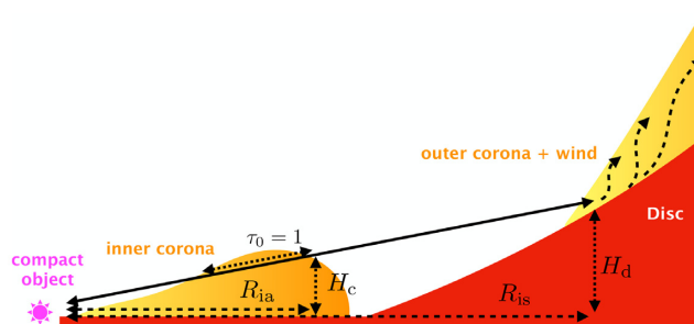
Figure 3. Schematic view of an inner corona and a wind.
