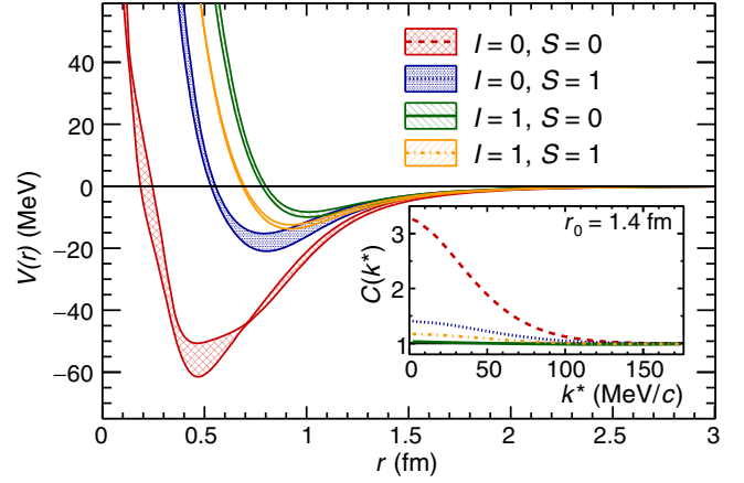
FIG. 2. Predictions for the \Xi -nucleon potential from the HAL-QCD Collaboration [42] for the different spin ( S ) and isospin ( I ) states. The error bands refer to different Euclidean times considered in the calculation. The inset shows the correlation function computed with the central value of the potential for each of the different states and a source radius of 1.4 fm.
