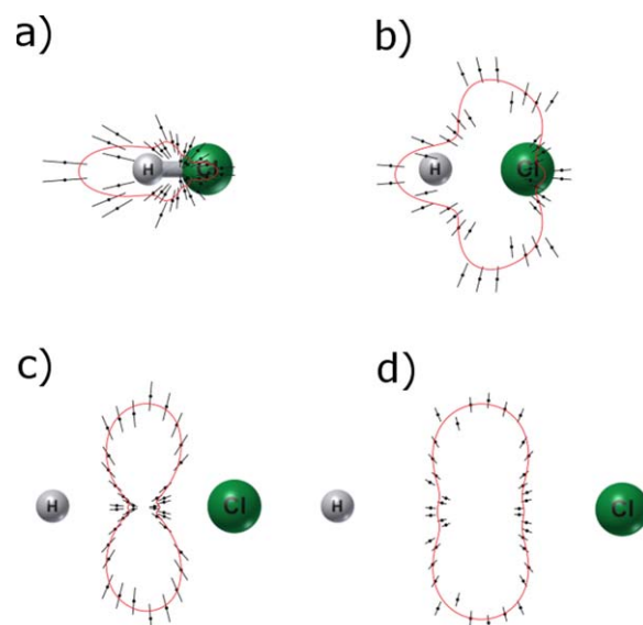
Figure 25. Auger electron angular distribution in the molecular frame as the HCl molecule undergoes the transition from (a) molecule to (d) separated atoms. Reprinted figure with permission from [177], Copyright 2016 by the American Physical Society.
