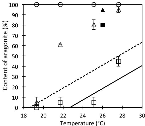
Figure 2. Aragonite content in Acropora cultured under different temperature and mMg/Ca regimes. Circle symbols— mMg/Ca = 5.2; open triangles— mMg/Ca = 1.0; open squares— mMg/Ca = 0.5, mean ± standard error ( n = 3) (all A. solitaryensis ; this study); solid triangle— mMg/Ca = 1.0; solid square— mMg/Ca = 0.5 (both A. tenuis ; Higuchi et al., 2014). Dashed line indicates mMg/Ca = 1.0; solid line indicates mMg/Ca = 0.5 [by linear regression model A = (T + 8.5 \times mMg/Ca - 26.6)/0.18 ( T is temperature); modified from Kiessling, 2015]. Plots above lines indicate higher proportion of aragonite skeleton than inorganic precipitation of aragonite.
