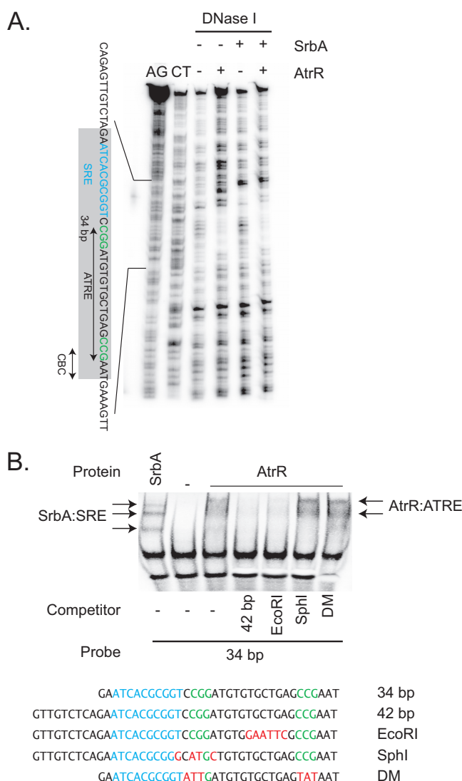
FIG 7 AtrR binding to cyp51A . (A) A 5'-end-labeled probe corresponding to the cyp51A promoter region was prepared and used in Maxam-Gilbert chemical sequencing reactions (AG, purine residues; CT, pyrimidine residues) to generate a size standard to allow localization of the binding sites for AtrR and SrbA. This same probe was then used in a standard DNase I protection assay with the addition of recombinant forms of AtrR or SrbA where indicated. The drawing on the left represents the sequence elements of interest. The gray bar denotes the bounds of the 34-bp region that is duplicated in the TR 34 promoter mutation. The double-headed arrow labeled CBC indicates the previously shown binding site for the CAAT-binding complex (9), and the sequence in blue represents a previously mapped SrbA response element (SRE) from this same earlier study. The AtrR response element (ATRE) is indicated with the two CCG repeats in green text. (B) Electrophoretic mobility shift assay (EMSA) analysis of sequence requirements for AtrR binding. A biotin-labeled form of the 34-bp element from cyp51A was used as a probe for all these EMSA reactions. Recombinant forms of SrbA or AtrR were added to this probe in the absence or presence of the indicated nonbiotinylated competitor DNAs listed at the bottom. Protein-DNA complexes formed by SrbA. The locations of the SRE and ATRE are shown as in panel A, with mutant residues indicated by red text. All competitors were present at 10-fold molar excess.
