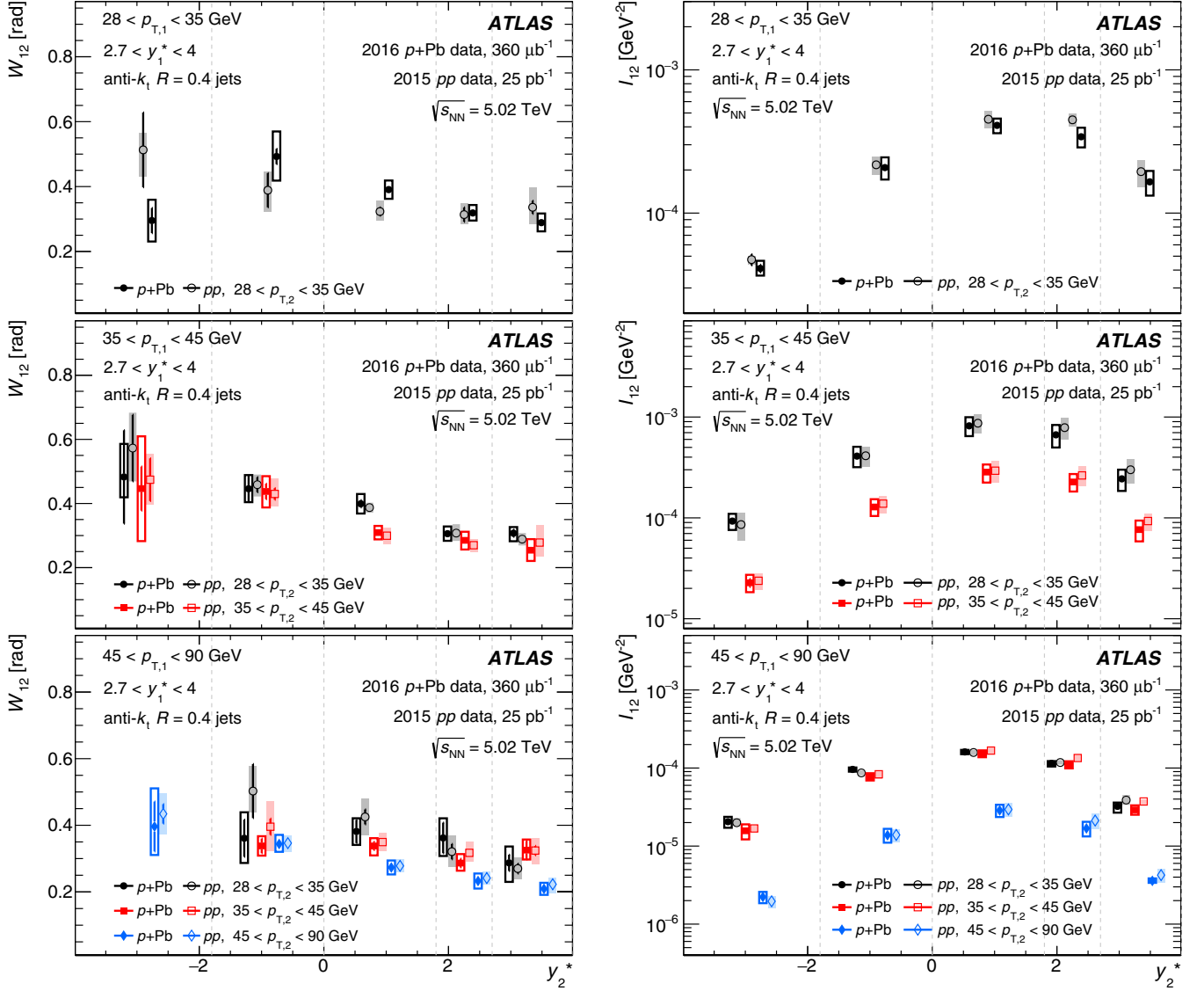
FIG. 5. Comparison of (left) W_{12} and (right) I_{12} values in pp (open symbols) and p + \text{Pb} (closed symbols) collisions for different selections of p_{T,1} and p_{T,2} as a function of y_2^* . The y_2^* intervals are separated by dotted vertical lines. The data points are shifted horizontally for visibility, and do not reflect an actual shift in rapidity. The vertical size of the shaded and open boxes represents systematic uncertainties for pp and p + \text{Pb} , respectively, and the error bars indicate statistical uncertainties. The horizontal size of the shaded and open boxes does not represent the width of the bins. Some points are not presented due to large statistical uncertainties. Results are shown with no \Delta p_T requirement, where \Delta p_T = p_{T,1} - p_{T,2} .
