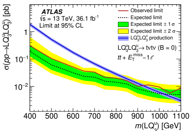
Figure 10. Observed and expected 95% CL upper limit on the cross-section for up-type LQ pair production with B = 0 as a function of the LQ mass. The \pm 1(2)\sigma uncertainty bands around the expected limit represent all sources of statistical and systematic uncertainties. The thickness of the theory curve represents the theoretical uncertainty from PDFs, renormalization and factorization scales, and the strong coupling constant \alpha_s .
