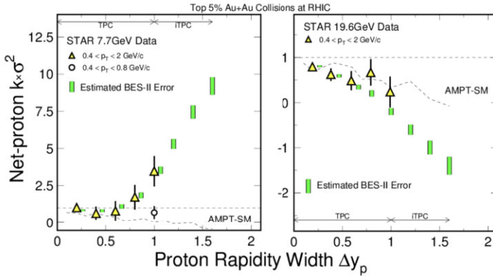
Fig. 1. The observed net-proton kurtosis times the variance as a function of the rapidity window from BES-I (yellow triangles) for Au+Au collisions at \sqrt{s_{NN}} = 7.7 GeV and 19.6 GeV. The green boxes represent the estimated statistical uncertainty for the BES-II program.
