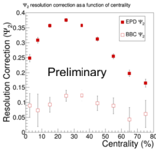
Fig. 3. An estimate of the second order event plane resolution at top energy Zr+Zr/Ru+Ru after azimuthal angle re-weighting to flatten the event plane for the EPD (solid square) and the BBC (open square).
