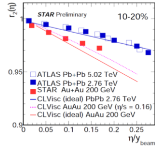
Fig. 4. Longitudinal de-correlation of elliptic anisotropy ( r_2 ) in Au+Au at \sqrt{s_{NN}} = 200 GeV using the existing FMS detector ( 2.5 < \eta < 4 ).
