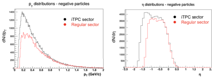
Fig. 2. Comparisons between reconstructed tracks for negatively charged particles in the iTPC and a regular sector. Left: raw p_T distribution, and Right: raw dN/d\eta distribution.
