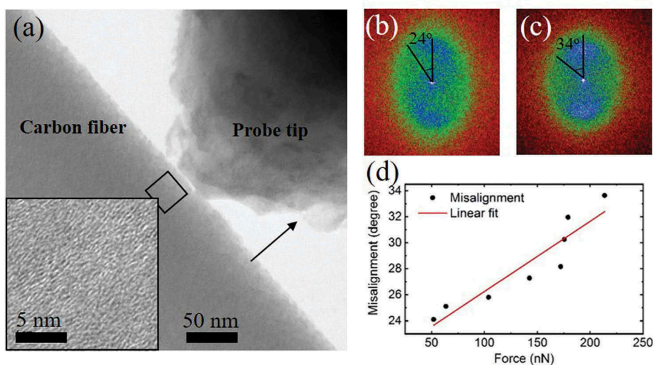
Figure 2. (a) Low magnification TEM image showing the AFM tip indenting on a specimen sliced from a CF. Inset shows high-resolution image about the indented region; (b,c) fast Fourier transform patterns of the same region as marked by the dark square in (a), where misalignment angle of graphene layers changed before and after the application of indenting force of 220 nN; (d) plot of misalignment angle with the applied indenting force to the CF specimen.
