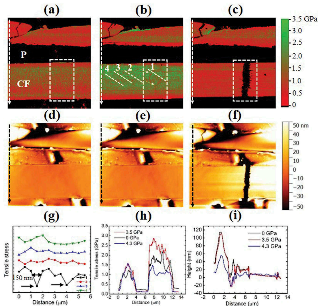
Figure 4. (a) Tensile stress map created in an area on CFRP containing a broken CF at the upper position and an intact CF at the lower position; (b) same region with applied external stress showing stress concentration on the lower intact CF and some newly formed defects; (c) fracture occurred at the lower CF when external tensile stress was further increased; (d–f) height map obtained simultaneously with modulus maps in (a–c); (g) modulus line profiles created at the position marked with 1–4 in (b), showing spatial resolution better than 150 nm at two defect locations; (h) modulus line profiles created along the white arrows in (a–c), respectively; (i) height line profiles created at the same position as in (h).
