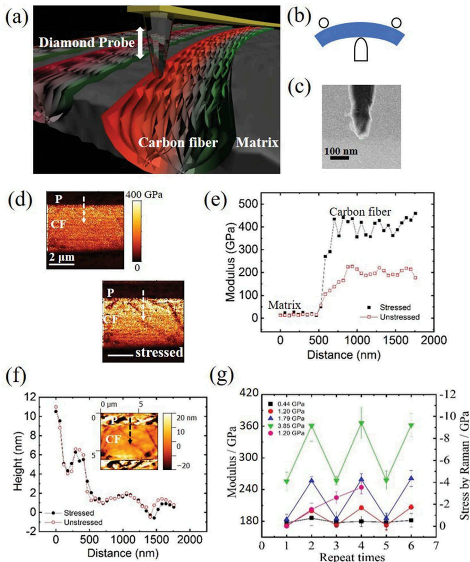
Figure 1. (a) Experimental principle showing the diamond tip indenting in the in-plane direction of graphene layers of a CF imbedded in polymer matrix; (b) schematics showing the three-point bending holder used to apply tensile stress to the CFRP specimen; (c) scanning helium ion microscopy image of the diamond tip after the experiment; (d) compressive modulus map of the same CF region with and without applied external tensile stress; (e) modulus line profiles created along the white arrows in (d) showing large modulus hardening of the stressed CF; (f) height line profiles created at the same positions as (e). Inset showing one height map of the same CF region; (g) indentation moduli obtained from a CF during cyclic tensile loading of four different average stresses with comparison to Raman spectroscopy measurements.
