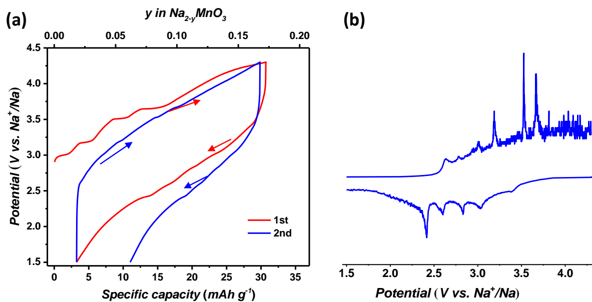
Figure S2. (a) The typical galvanostatic potential curves of \text{Na}_2\text{MnO}_3 for the initial two cycles at the current density of 10 \text{ mA g}^{-1} . (b) The corresponding dQ/dV curves with the second cycle derived from (a).
