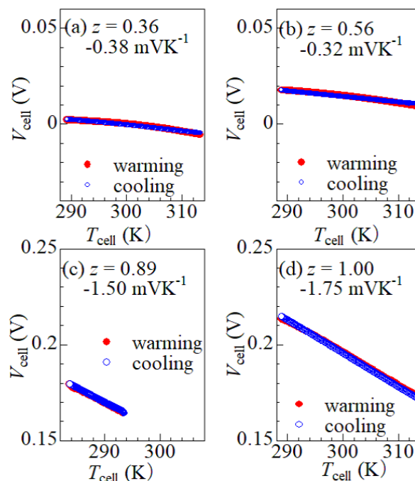
Fig. 2: Cell voltage ( V_{\text{cell}} ) of the NCF90/ \text{Co}_{1-z}\text{Mn}_z\text{-PBA} cell against the cell temperature ( T_{\text{cell}} ); (a) z = 0.36 , (b) 0.56, (c) 0.89, and (d) 1.00. Both the anode and cathode were the x -controlled films to the middle point of the low-V plateau. Red and blue marks mean that the data obtained in the heating and cooling runs, respectively.
