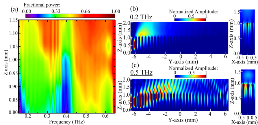
Fig. 4. (a) Frequency-dependent modal power fraction of the 30-layer MRA waveguide ( G_x=G_y=0.26 mm). Electric field distributions of (b) 0.2 and (c) 0.5 THz waves in the Y-Z and X-Z planes.
