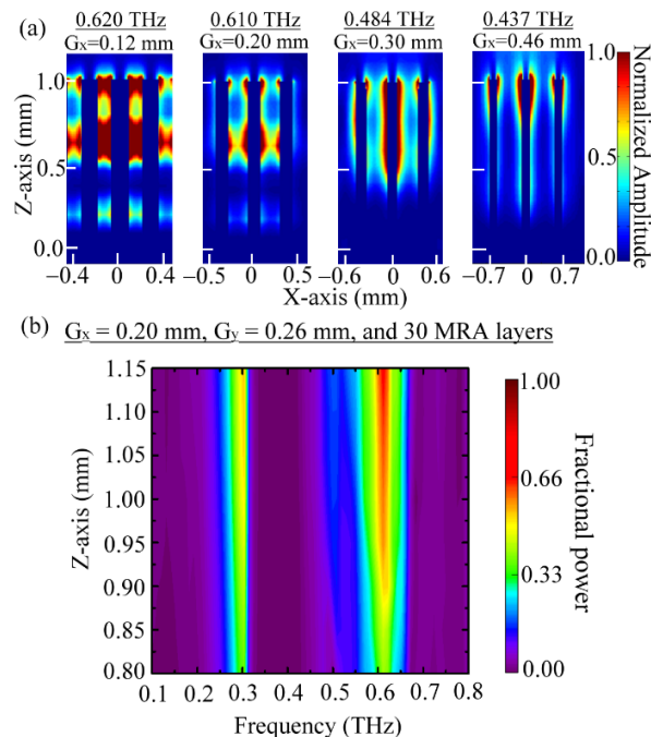
Fig. 7. (a) Electric field distributions at the 30th MRA layer for the transmission peaks of the 2nd TM modes dependent on G_x . (b) Frequency-dependent modal power fraction of the 30-layer MRA waveguide ( G_x=0.20 mm, G_y=0.26 mm).
