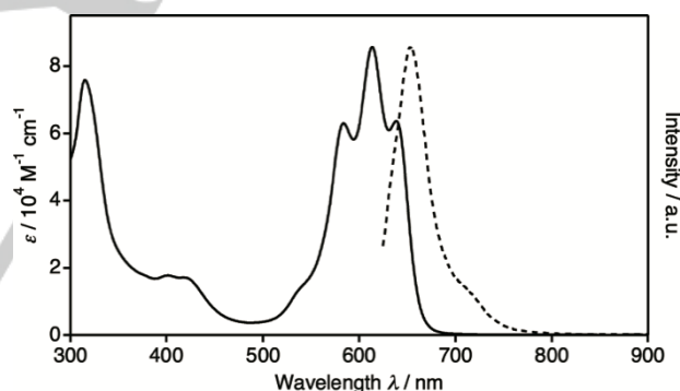
Figure 3. UV-vis absorption (solid line) and emission (dashed line) spectra of [\text{LBGa}(\text{CH}_3\text{OH})_2] in toluene/ \text{CH}_3\text{OH} = 95/5 (v/v) ( \lambda_{\text{ex}} = 614 \text{ nm} ).
