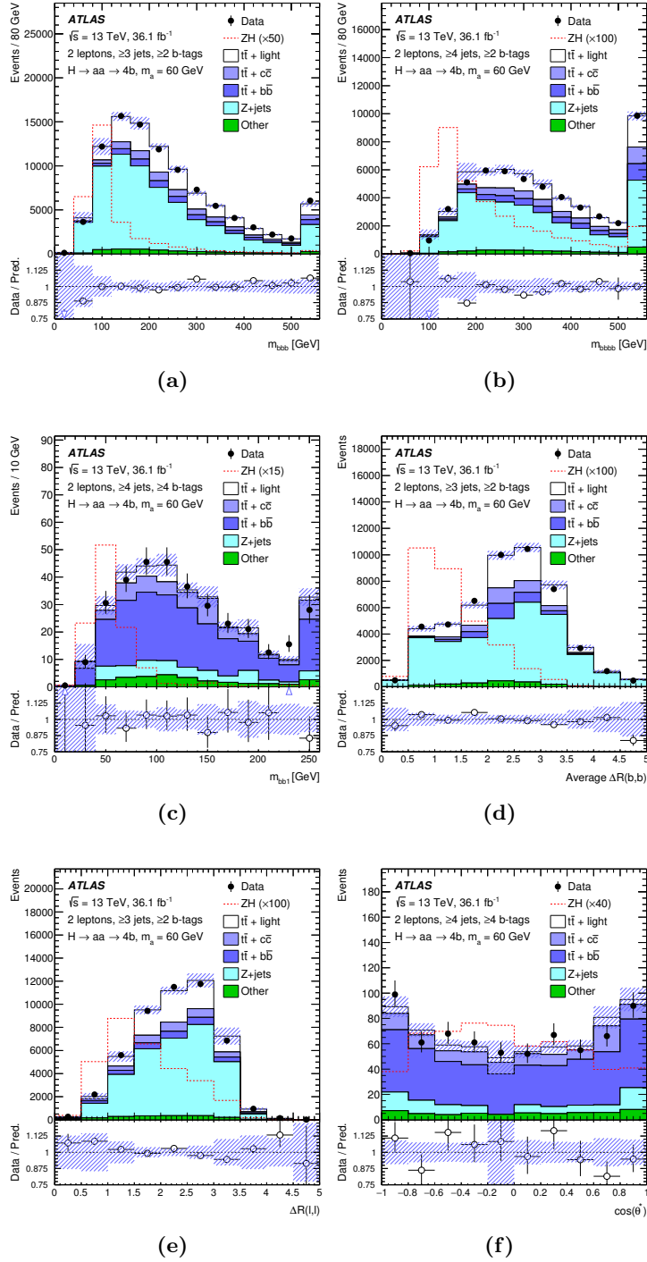
Figure 5. Comparison of data with the post-fit background estimates for (a) m_{bbb} , (b) m_{bbbb} , (c) m_{bb1} , (d) average \Delta R(b,b) , (e) \Delta R(\ell,\ell) and (f) \cos\theta^* in the dilepton sample inclusive in number of jets and b -tagged jets. Comparisons use events with \geq 3 jets, except when \geq 4 jets are necessary to define the variable, in which case events with \geq 4 jets are used. Distributions for the signal model ( ZH , H \rightarrow aa \rightarrow 4b ), with m_a = 60 GeV, normalized to the SM pp \rightarrow ZH cross-section, assuming \mathcal{B}(H \rightarrow aa \rightarrow 4b) = 1 and scaled by a factor as indicated in the figure, are overlaid. The hashed area represents the total uncertainty in the background. The last bin contains the overflow.
