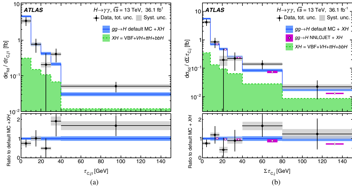
FIG. 38. The differential cross sections for pp \rightarrow H \rightarrow \gamma\gamma as a function of (a) \tau_{C_{j1}} and (b) \sum \tau_{C_j} are shown and compared to the SM expectations. The data and theoretical predictions are presented in the same way as in Fig. 36. In addition, the NNLOJET prediction is displayed in (b).
