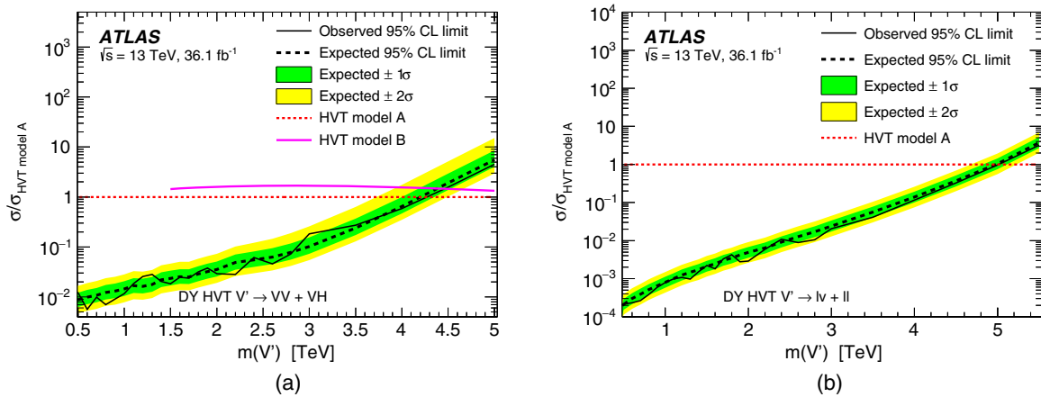
FIG. 7. Observed and expected 95% C.L. upper limits on the V' cross section times branching fraction to (a) VV/VH and (b) l\nu/l\ell for the HVT benchmark model, relative to the cross section for HVT model A. The model predictions are also shown.
