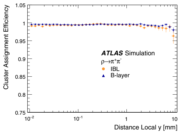
(a) \rho \rightarrow \pi^+ \pi^- sample
