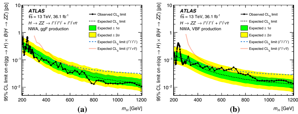
Fig. 6 The upper limits at 95% CL on the cross section times branching ratio as a function of the heavy resonance mass m_H for a the ggF production mode ( \sigma_{ggF} \times B(H \rightarrow ZZ) ) and b for the VBF production mode ( \sigma_{VBF} \times B(H \rightarrow ZZ) ) in the case of the NWA. The green and
