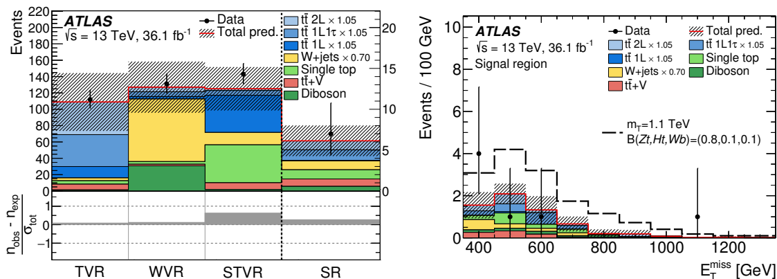
Figure 5. Left panel: comparison of the observed data ( n_{\text{obs}} ) with the predicted background ( n_{\text{exp}} ) in the VRs and SR. The bottom panel shows the significance of the difference between data and predicted background, where the significance is based on the total uncertainty ( \sigma_{\text{tot}} ). Right panel: comparison of data and prediction in the E_T^{\text{miss}} distribution in the SR. The error bands include statistical and systematic uncertainties. The expected shape for a signal with m_T = 1.1 TeV and B(T \rightarrow Zt) = 80\% is added on top of the SM prediction.
