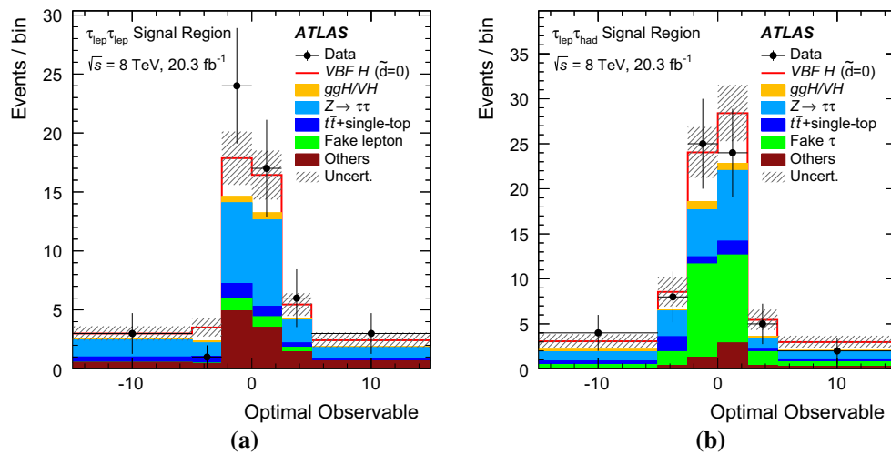
Fig. 5 Distributions of the Optimal Observable in the signal region for the a \tau_{lep}\tau_{lep} and b \tau_{lep}\tau_{had} channel, after the global fit performed for the \tilde{d} = 0 hypothesis. The best-fit signal strength is \mu = 1.55^{+0.87}_{-0.76} . The
