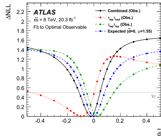
Fig. 6 Observed and expected \Delta NLL as a function of the \tilde{d} values defining the underlying signal hypothesis, for \tau_{lep}\tau_{lep} (green), \tau_{lep}\tau_{had} (red) and their combination (black). The best-fit values of all nuisance parameters from the combined fit at each \tilde{d} point were used in all cases. An Asimov dataset with SM backgrounds plus pure CP-even VBF signal ( \tilde{d} = 0 ), scaled to the best-fit signal-strength value, was used to calculate the expected values, shown in blue. The markers indicate the points where an evaluation was made – the lines are only meant to guide the eye
