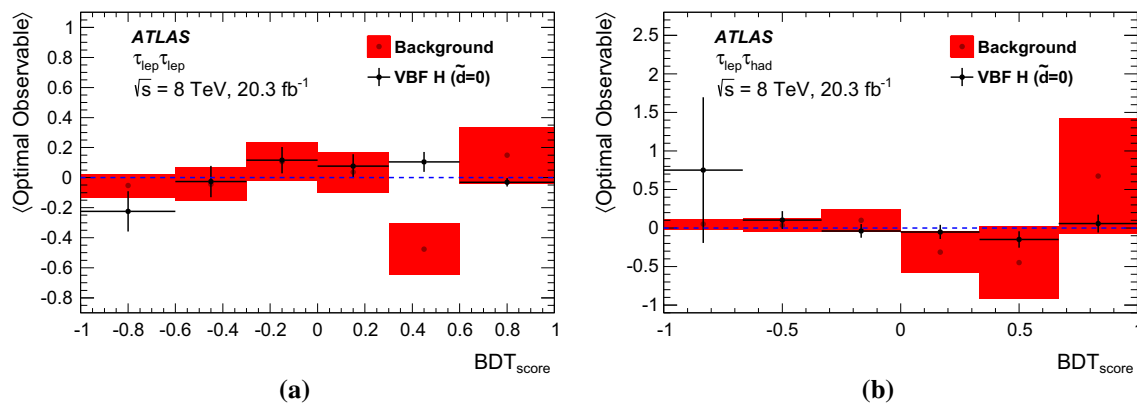
Fig. 2 Mean of the Optimal Observable as a function of the \text{BDT}_{\text{score}} for the SM signal ( black dots with error bars ) and for the sum of all background processes ( filled red area ), for the a \tau_{\text{lep}}\tau_{\text{lep}}
