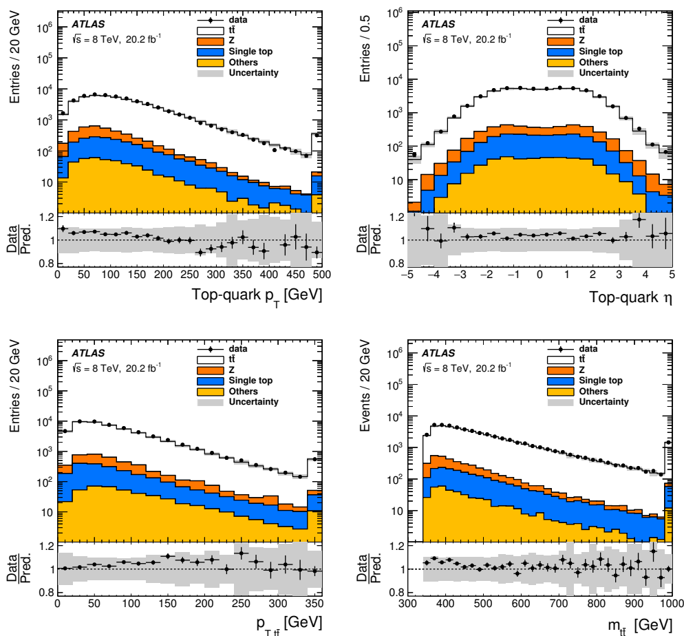
Figure 2. Comparison between data and predictions after the kinematic reconstruction in the combined dilepton channel. The distributions of the top quark p_T and \eta are shown, as well as the t\bar{t} p_T and mass. The ratio between the data and prediction is also shown. The grey area shows the statistical and systematic uncertainty on the signal and background. The t\bar{t}V , diboson and fake-lepton backgrounds are shown together in the “Others” category. The last bin of the distribution corresponds to the overflow.
