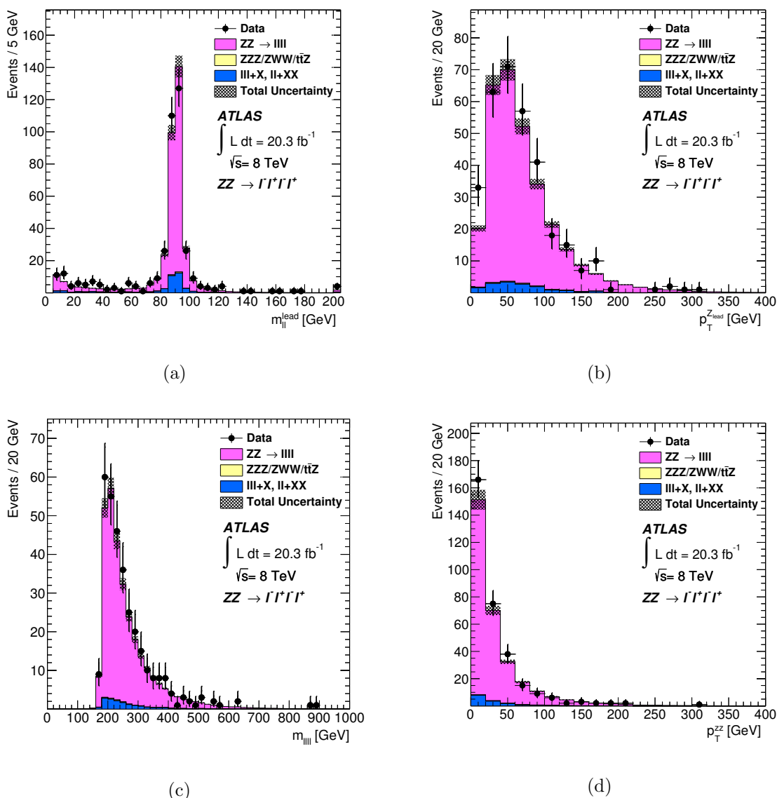
Figure 2. Kinematic distributions for ZZ \rightarrow \ell^- \ell^+ \ell'^- \ell'^+ candidates in all four-lepton final states: (a) m_{\ell^- \ell^+}^{\text{lead}} , (b) p_T^{Z\text{lead}} , (c) m_{\ell^- \ell^+ \ell'^- \ell'^+} and (d) p_T^{ZZ} . The points represent the observed data and the histograms show the expected number of ZZ signal events and the background estimate. The shaded band shows the combined statistical and systematic uncertainties in the prediction and the background. No selection on the leading lepton pair mass is required for (a), while the full selection is applied for the other distributions.
