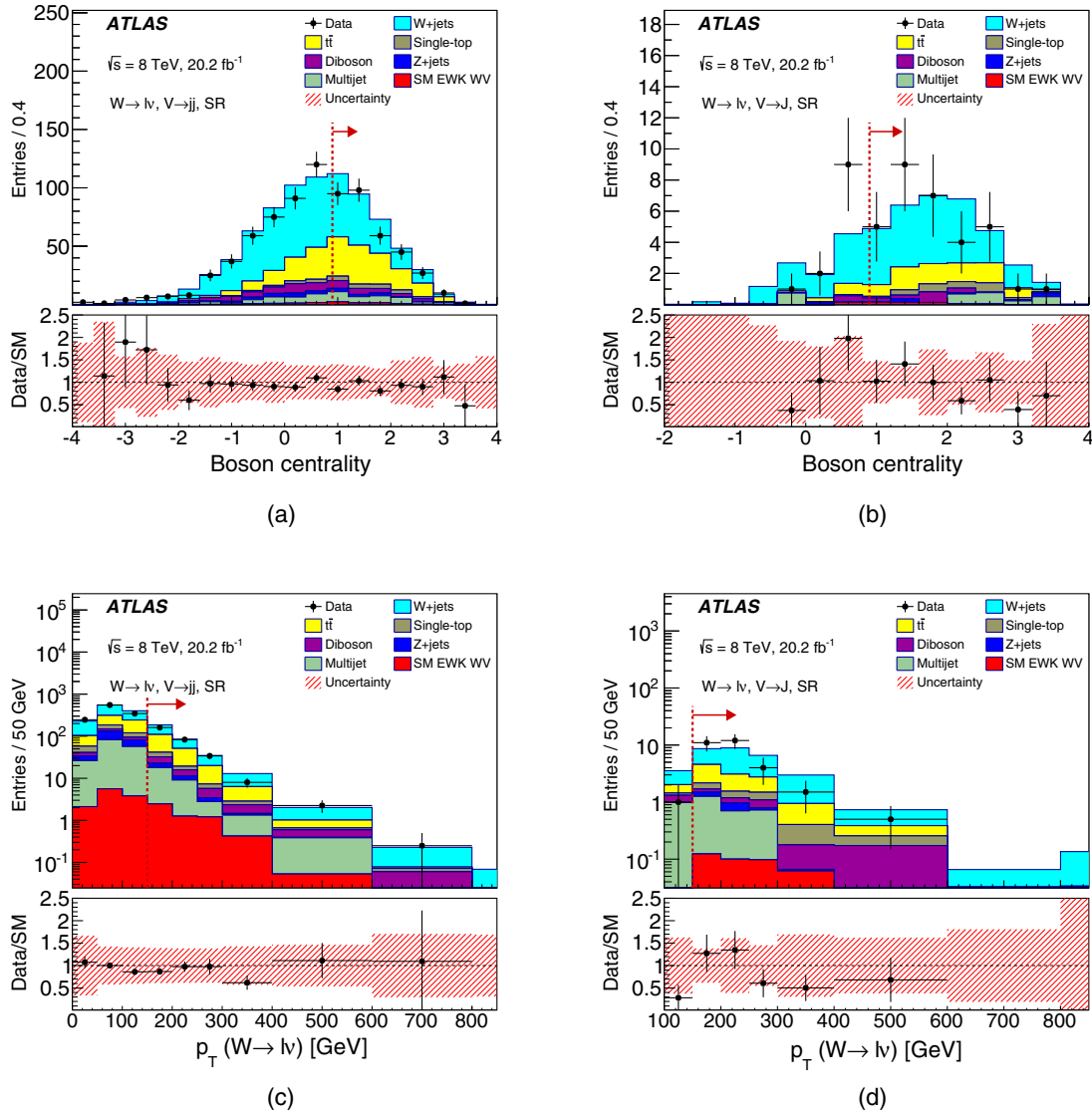
FIG. 3. The observed boson centrality (top) and p_T(W_{\text{lep}}) (bottom) distributions, compared to the SM prediction. Plots (a) and (c) show the resolved ( V \rightarrow \text{jj} ) signal region (SR), and plots (b) and (d) show the merged ( V \rightarrow \text{J} ) signal region, except that the \zeta_V > 0.9 requirement is not applied for the boson centrality plots, and the p_T(W_{\text{lep}}) > 150 GeV requirement is not applied for the p_T(W_{\text{lep}}) plots. The red vertical lines and arrows indicate the signal region selection. The last bin includes overflow.
