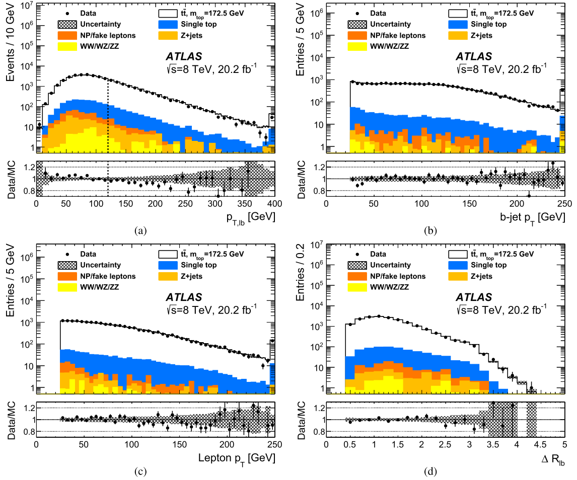
Fig. 1. Kinematic distributions obtained from the objects assigned to the two lepton– b -jet pairs for (a) the pre-selection, or (b)–(d) the final selection. The average p_{T} of the two lepton– b -jet pairs, denoted by p_{T,lb} , is shown in (a). The p_{T,lb} requirement for the final selection is indicated by the vertical dashed line. The remaining distributions show the p_{T} of the b -jets in (b), the p_{T} of the leptons in (c), and the \Delta R_{lb} of the lepton and the b -jet for the two lepton– b -jet pairs in (d). The rightmost bin contains the overflow, if present. For all distributions, the number of predicted events is normalised to the one observed in the data. The hatched area corresponds to the statistical uncertainties in the prediction, the uncertainty bars to the statistical uncertainties in the data. For each figure, the ratio of data and prediction is also presented.
