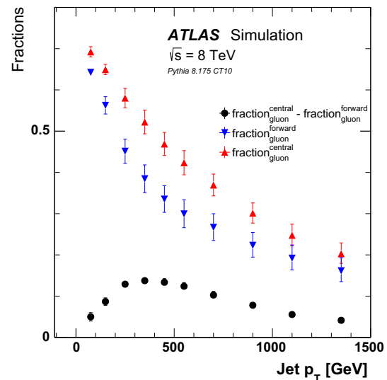
Fig. 2 The simulated fraction of jets originating from gluons as a function of jet p_T for the more forward jet ( down triangle ), the more central jet ( up triangle ), and the difference between these two fractions ( circle ). The fractions are derived from PYTHIA 8 with the CT10 PDF set and the error bars represent the PDF and matrix element uncertainties, further discussed in Sect. 6. The uncertainties on the fraction difference are computed from propagating the uncertainties on the more forward and more central fractions, treating as fully correlated
