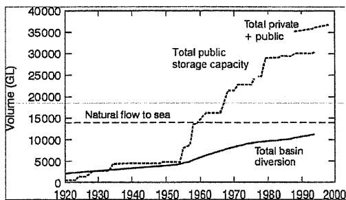
Figure 3. Storage capacity and diversions in the Murray-Darling Basin from 1920 to 2000.
