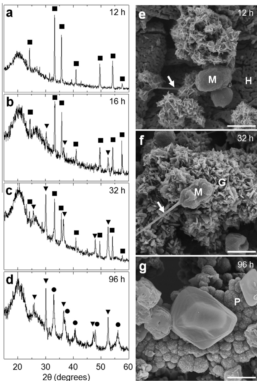
Fig. 3. Changes in minerals during cultivation. M. jannaschii was cultured in Mc + S 0 + hematite medium for the designated periods. The sediments were analyzed by XRD (a–d) and FE-SEM (e–g). Greigite, closed triangles. Hematite, closed squares. Pyrite, closed circles. The broad peak around 2\theta = 20^\circ was derived from the polyimide film. The ordinate shows arbitrary signal intensity. A dividing M. jannaschii cell (M), as inferred from the cell shape, and an accompanying bridge (arrow) made from flagella (Igarashi and Kuwabara, 2014); hematite (H); greigite-like nanoflakes (G); and framboidal pyrite-like botryoids (P). Bars: 1 \mu\text{m} .
