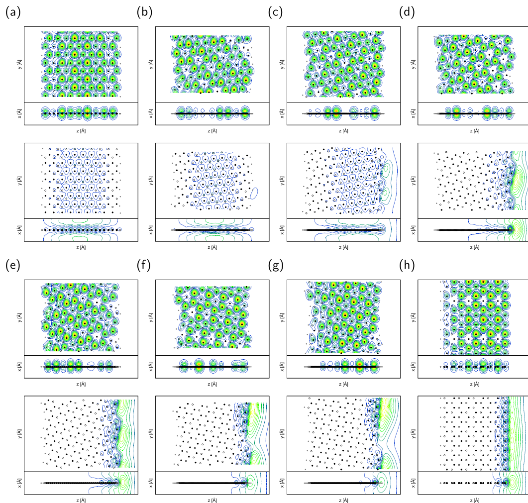
Figure 5. Wave functions of hydrogenated h-BN nanoribbons. Top ( x = 0 ) and side ( y = 0 ) views of contour plots of wave functions at the \Gamma point near the Fermi level E_F of hydrogenated h-BN nanoribbons with edge angles \theta of (a) 0^\circ , (b) 5^\circ , (c) 8^\circ , (d) 14^\circ , (e) 16^\circ , (f) 22^\circ , (g) 23^\circ , and (h) 30^\circ . In each figure, upper and lower panels denote VBT and CBB states, respectively. Black, white, and gray circles denote the atomic positions of nitrogen, boron, and hydrogen atoms, respectively.
