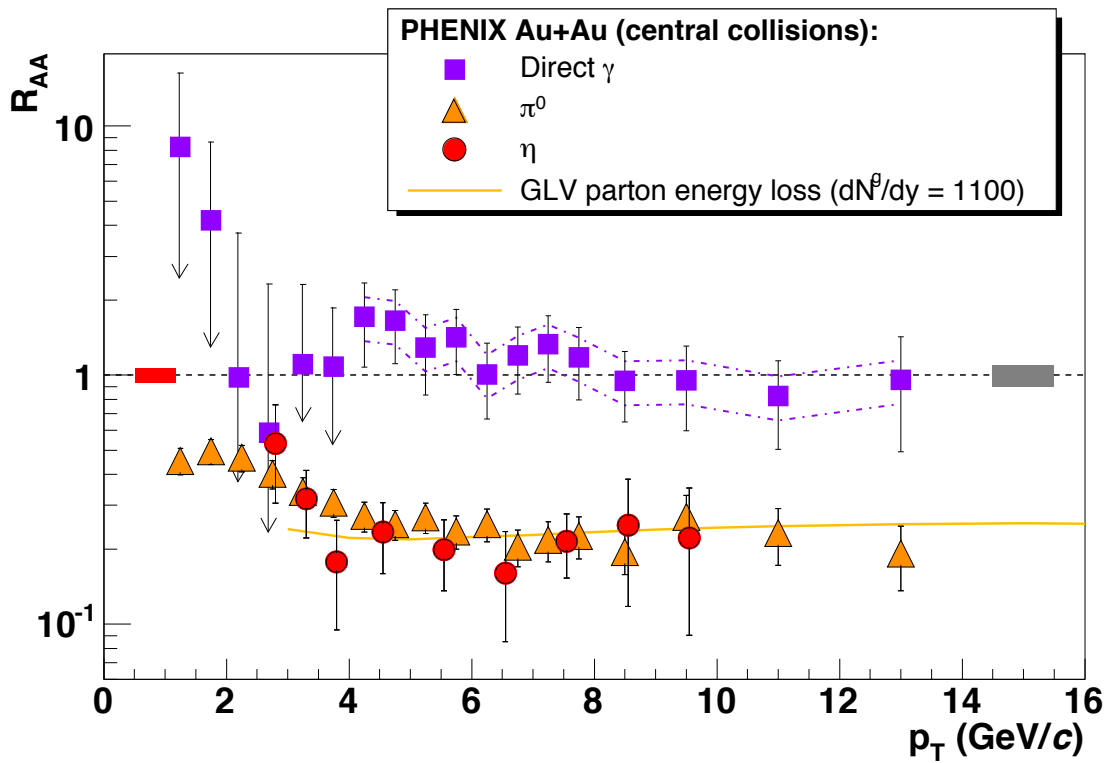
Fig. 1.6.1: Nuclear modification factors of \pi^0 , \eta , direct \gamma as functions of p_T in central Au+Au collisions at \sqrt{s_{NN}} = 200 GeV/c[22]. The solid yellow curve is a parton energy loss prediction for a medium with density dN^g/dy = 1100 .
