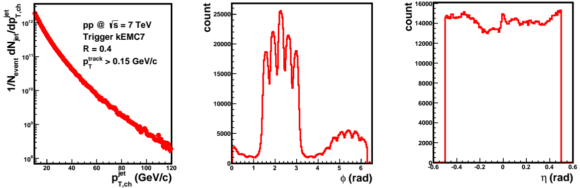
Fig. 3.4.2: Charged jet p_T , \phi end \eta distributions with R=0.4 , A_{area} > 0.4 and input track p_T^{track} > 0.15 (GeV/c), used EMCal triggered events.
