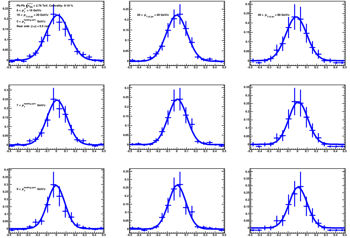
Fig. 4.3: Near side peaks in |\Delta\phi| < 0.5 (rad) fitted by Gaussian functions in Pb-Pb collisions at \sqrt{s_{NN}} = 2.76 TeV with trigger \pi^0 momentum region 8 < p_T^{\pi^0} < 16 GeV/c. The momentum ranges of the associated jets increase with going to right sides and the momentum thresholds of the leading particle in a jet increase with going bottom sides.
