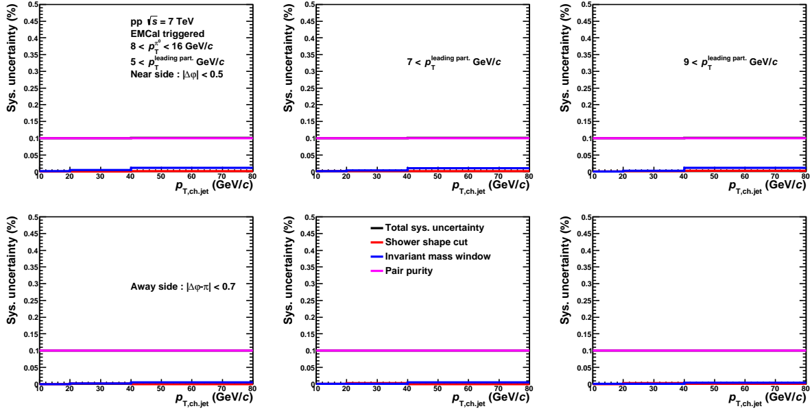
Fig. 5.6.7: The systematic uncertainties as a function of jet p_{T,ch,jet} for near (top) and away (bottom) side RMSs in pp collisions with the momentum range of trigger \pi^0 8 < p_T^{\pi^0} < 16 GeV/c. The momentum thresholds of leading particle in a jet 5(left), 7(center), 9(right) < p_T^{leadingpart} . GeV/c.
