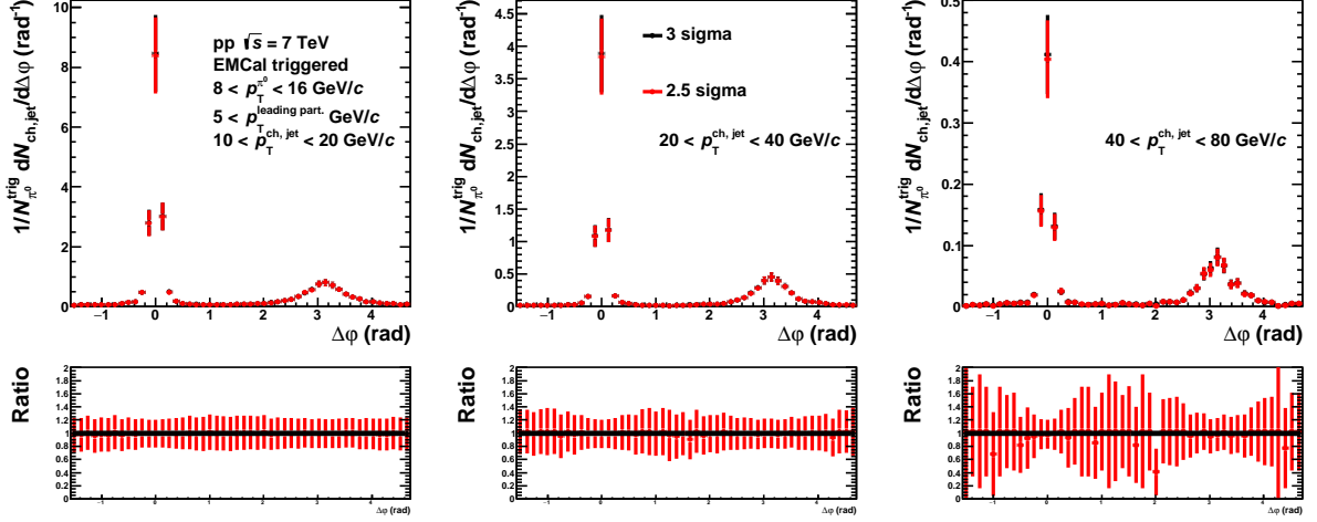
Fig. 5.2.1: Comparison of the two kinds of invariant mass (black:3 sigma, red:2.5 sigma) cuts of azimuthal correlations (top) and its ratios (bottom) in pp collisions with the momentum range of trigger \pi^0 8 < p_T^{\pi^0} < 16 GeV/c and associated jets 10 < p_{T,ch,jet} < 20 , 20 < p_{T,ch,jet} < 40 and 40 < p_{T,ch,jet} < 80 GeV/c. The momentum threshold of leading particle in a jet 5 < p_T^{leading part.} GeV/c.
