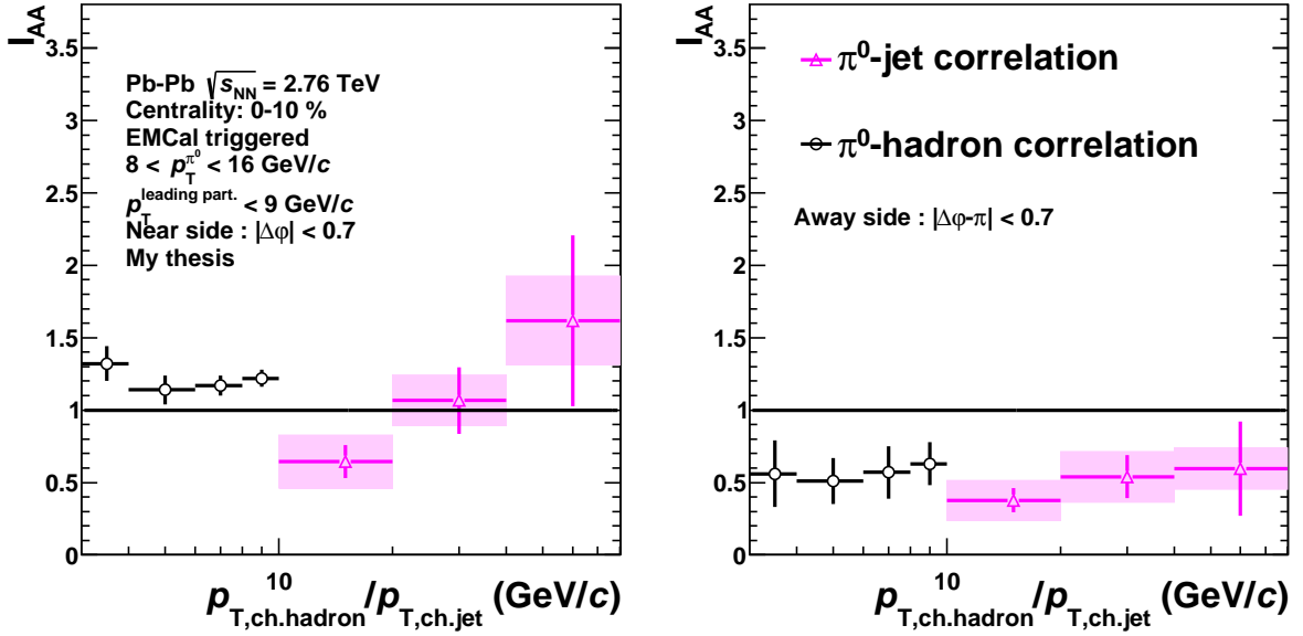
Fig. 6.3.2: Comparison of the ratio of per trigger yields I_{AA} as a function of the associated jet p_{T, \text{ch, jet}} between \pi^0 -charged hadron analysis (black) in the associated charged hadron p_T region 3 < p_{T, \text{ch.}} < 10 \text{ GeV/c} and \pi^0 -charged jet analysis (magenta) in the associated jet p_T region 10 < p_{T, \text{ch, jet}} < 80 \text{ GeV/c} with the p_T threshold of the leading particle in a jet p_T^{\text{leading part.}} > 9 \text{ GeV/c} .
