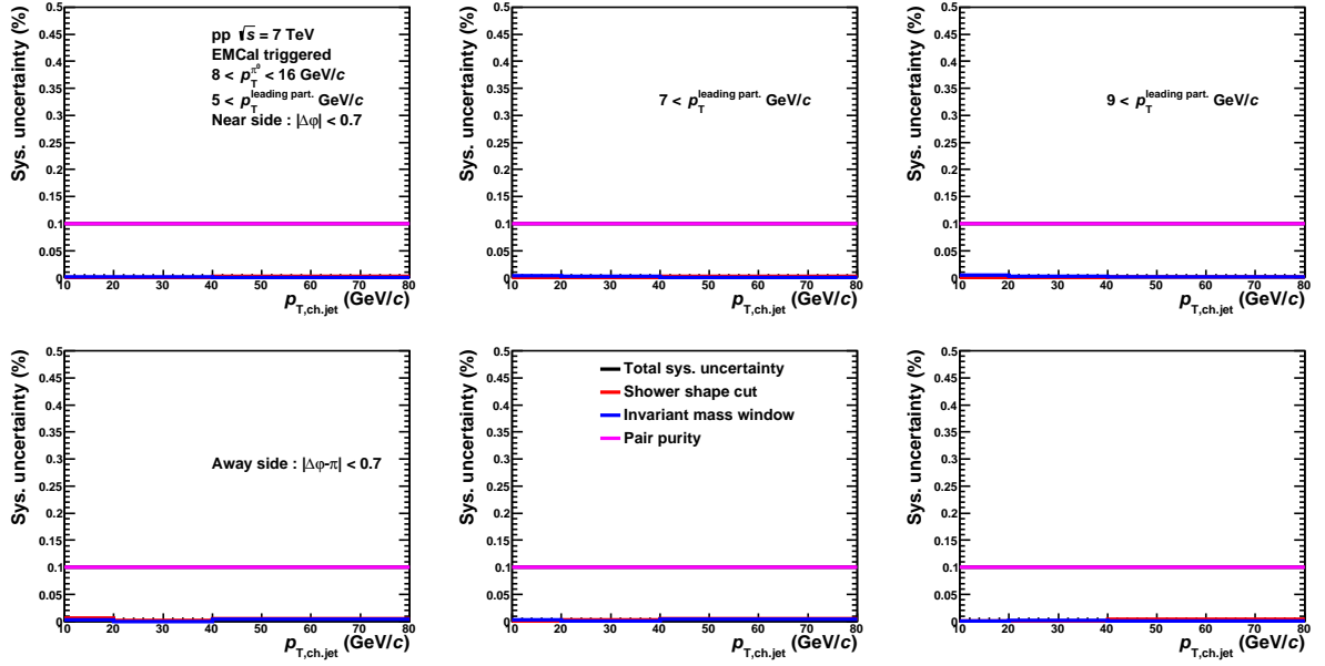
Fig. 5.6.5: The systematic uncertainties as a function of jet p_{T,ch,jet} for near (top) and away (bottom) side widths in pp collisions with the momentum range of trigger \pi^0 8 < p_T^{\pi^0} < 16 \text{ GeV}/c . The momentum thresholds of leading particle in a jet 5(left), 7(center), 9(right) < p_T^{leadingpart.} \text{ GeV}/c .
