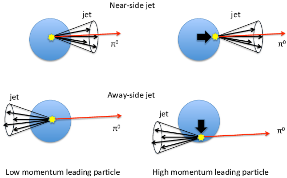
Fig. 1.8.3: Momentum dependence of the leading particle in a jet of the surface bias in near (top) and away-side (bottom). The left two figures are required a low momentum leading particle, the right figures are required a high momentum leading particle.
