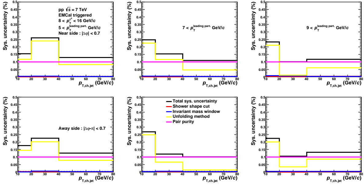
Fig. 5.6.3: The systematic uncertainties as a function of jet p_{T,ch,jet} for near (top) and away (bottom) side jet yields in pp collisions with the momentum range of trigger \pi^0 8 < p_T^{\pi^0} < 16 \text{ GeV}/c . The momentum thresholds of leading particle in a jet 5(left), 7(center), 9(right) < p_T^{\text{leading part.}} \text{ GeV}/c .
