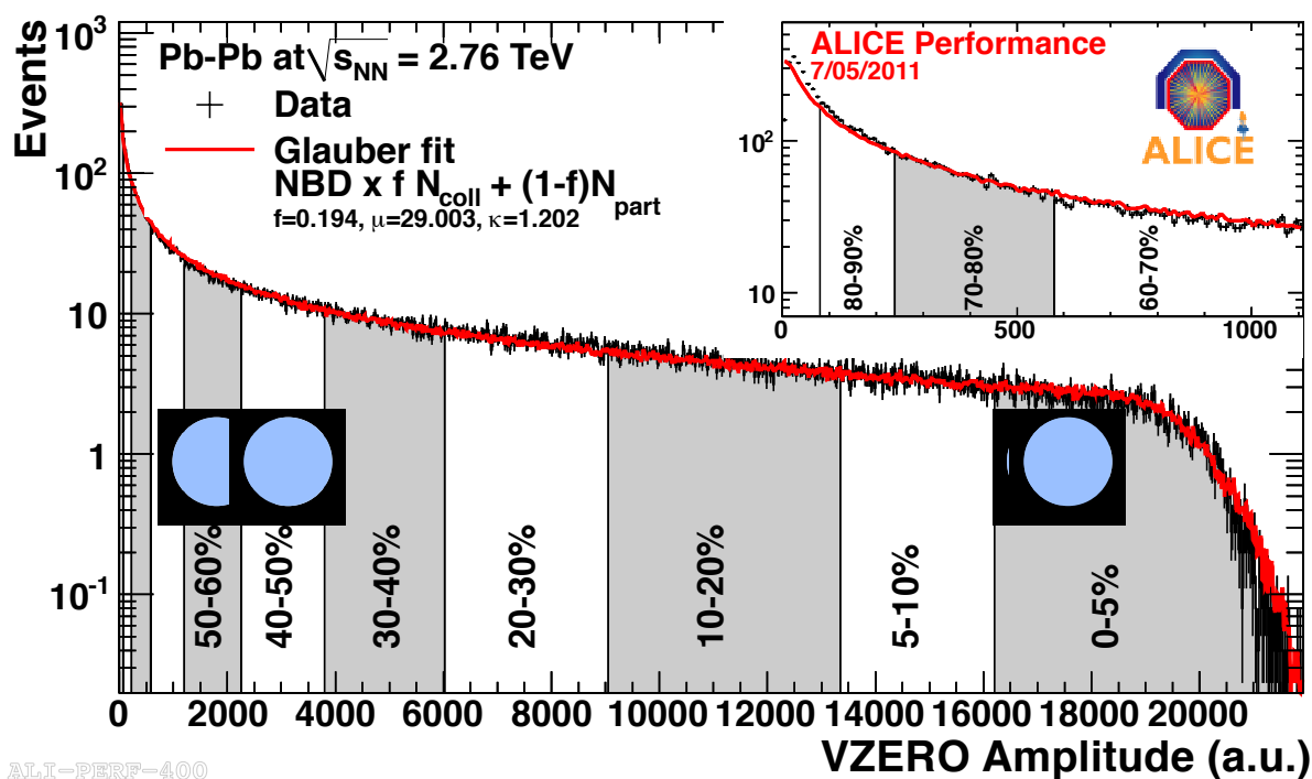
Fig. 3.2.2: V0 amplitude distribution with data and Glauber fitting.
