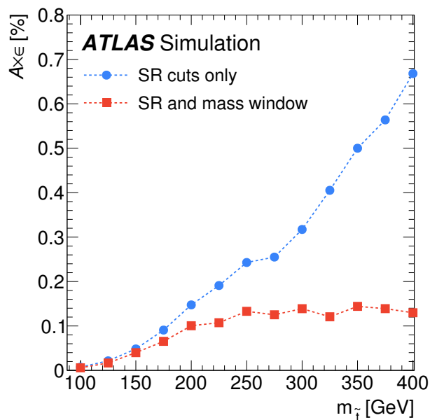
Figure 5. Total acceptance times efficiency ( A \times \epsilon ) of the SR cuts of eq. (5.3), and SR cuts combined with the mass window selection in table 1, as a function of m_{\tilde{t}} . The denominator of the efficiency (in %) is the total number of events, i.e. the top row in table 3.
