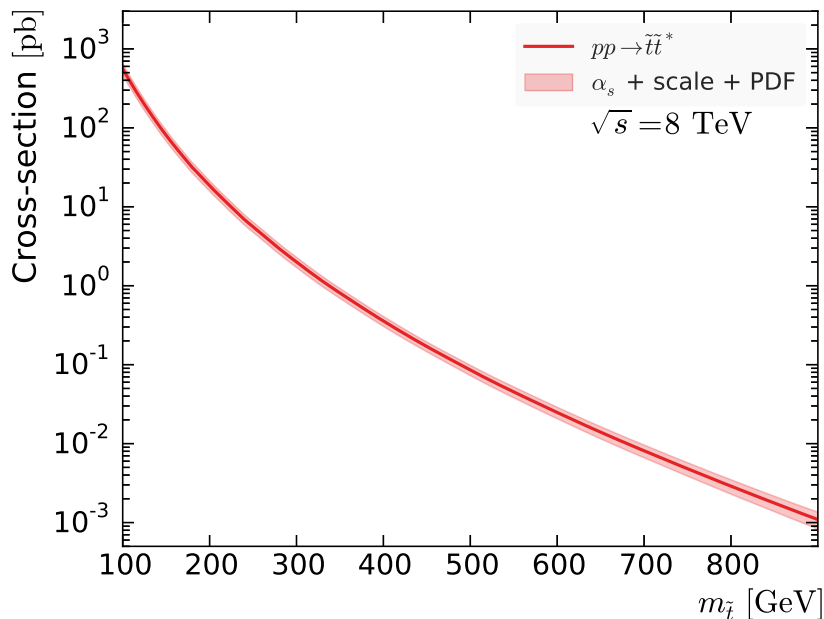
Figure 2. Cross-section for direct t\bar{t}^* pair production at the LHC centre-of-mass energy of \sqrt{s} = 8 TeV [63–65].
