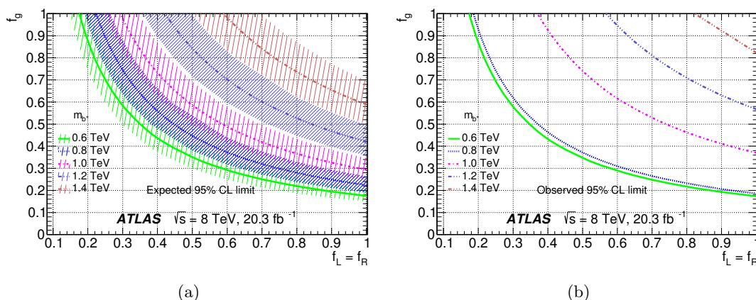
Figure 13. Expected (a) and observed (b) limit contours at the 95% CL as a function of the coupling parameters for several choices of m_{b^*} . The surrounding shaded bands correspond to \pm 1 standard deviations around the expected limits. For a given mass, couplings above the corresponding contour line are excluded.
