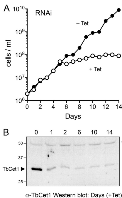
FIG 1 RNAi knockdown of TbCet1 arrests growth of T. brucei . (A) Procyclic T. brucei 29.13-TbCet1RNAi transfectants were inoculated into medium containing 1.0 \mu g/ml tetracycline (+Tet) to induce TbCet1 dsRNA production and into a parallel control culture lacking tetracycline (–Tet). Cell density was monitored by microscopy and maintained between 1 \times 10^6 and 1 \times 10^7 cells/ml by dilution into fresh medium. The growth curves display on the y axis the log of the direct cell count multiplied by the dilution factor. Induction of RNAi against TbCet1 arrested T. brucei growth after 5 days. (B) Western blotting verifies knockdown of TbCet1 protein by RNAi induction. An anti-TbCet1 immunoblot assay of total protein from cells harvested from a +Tet culture is shown. The positions and sizes (kilodaltons) of marker polypeptides are indicated on the left. The immunoreactive TbCet1 polypeptide, denoted by the arrowhead at left, is depleted after RNAi induction. A nonspecific cross-reacting 50-Da polypeptide, indicated by the asterisk at right, is unchanged.
