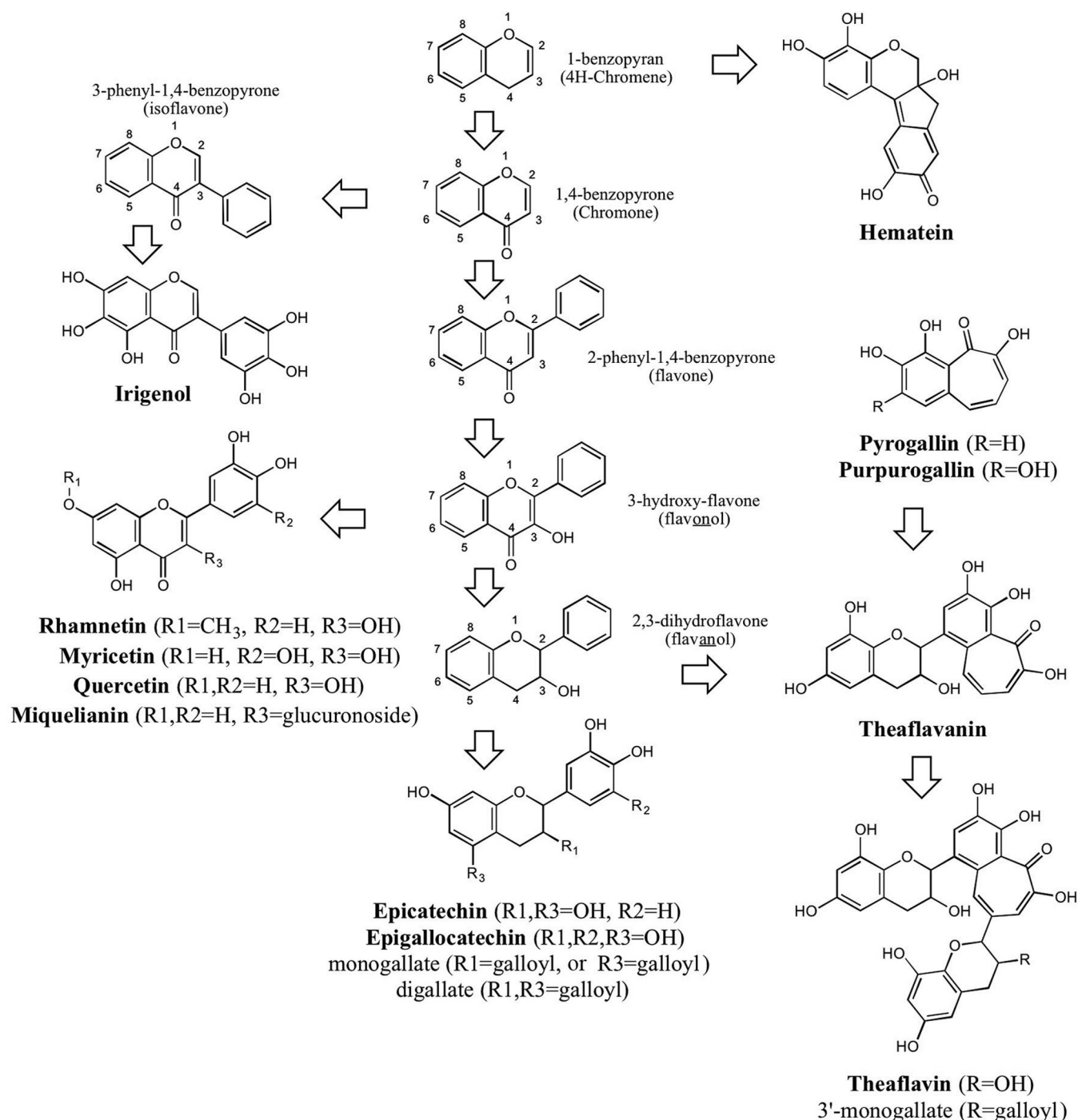
FIG 2 Chemical structures of flavonoid TbCet1 inhibitors and related compounds. Core scaffolds of flavonoids are labeled in lightface. TbCet1 inhibitors identified in the present study are labeled in boldface (with R groups in parentheses as specified). Arrows signify progressive chemical modifications.
