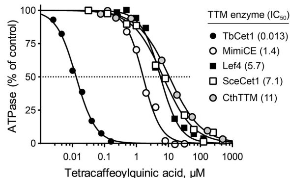
FIG 5 Tetra-caffeoylquinic acid activity against five TTM family ATPases. Dose-response profiles for tetra-caffeoylquinic acid inhibition of the indicated TTM enzymes. IC 50 s (μM) are indicated in parentheses.
