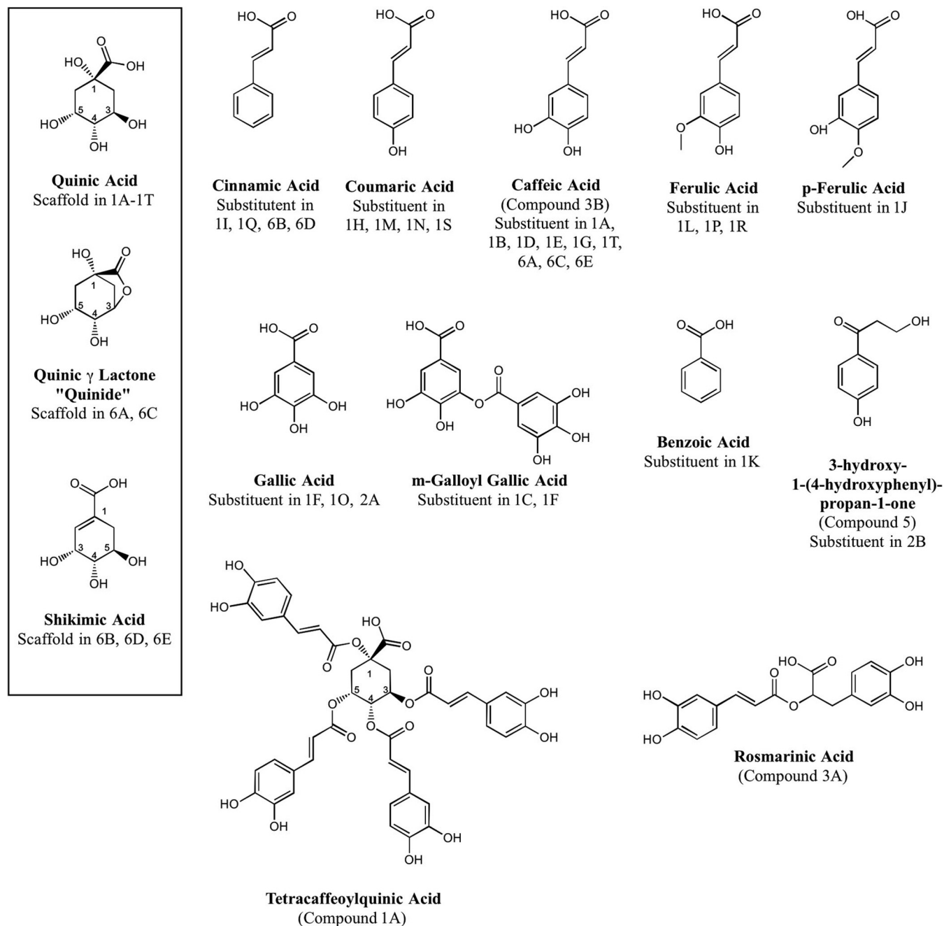
FIG 3 Chemical structures of chlorogenic acid TbCet1 inhibitors and related compounds. Core scaffolds of quinic acid, quinide, and shikimic acid are depicted in the box at left. Nine substituents esterified to the scaffolds are shown in the top and middle rows. The structures of tetracaffeoylquinic acid and rosmarinic acid are shown at bottom.
