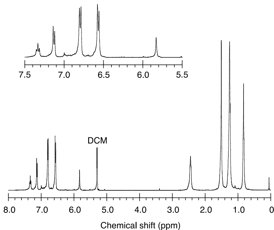
Figure 1-3. 1 H NMR spectrum of P3FT homopolymer (400 MHz in CD 2 Cl 2 at 298 K).
