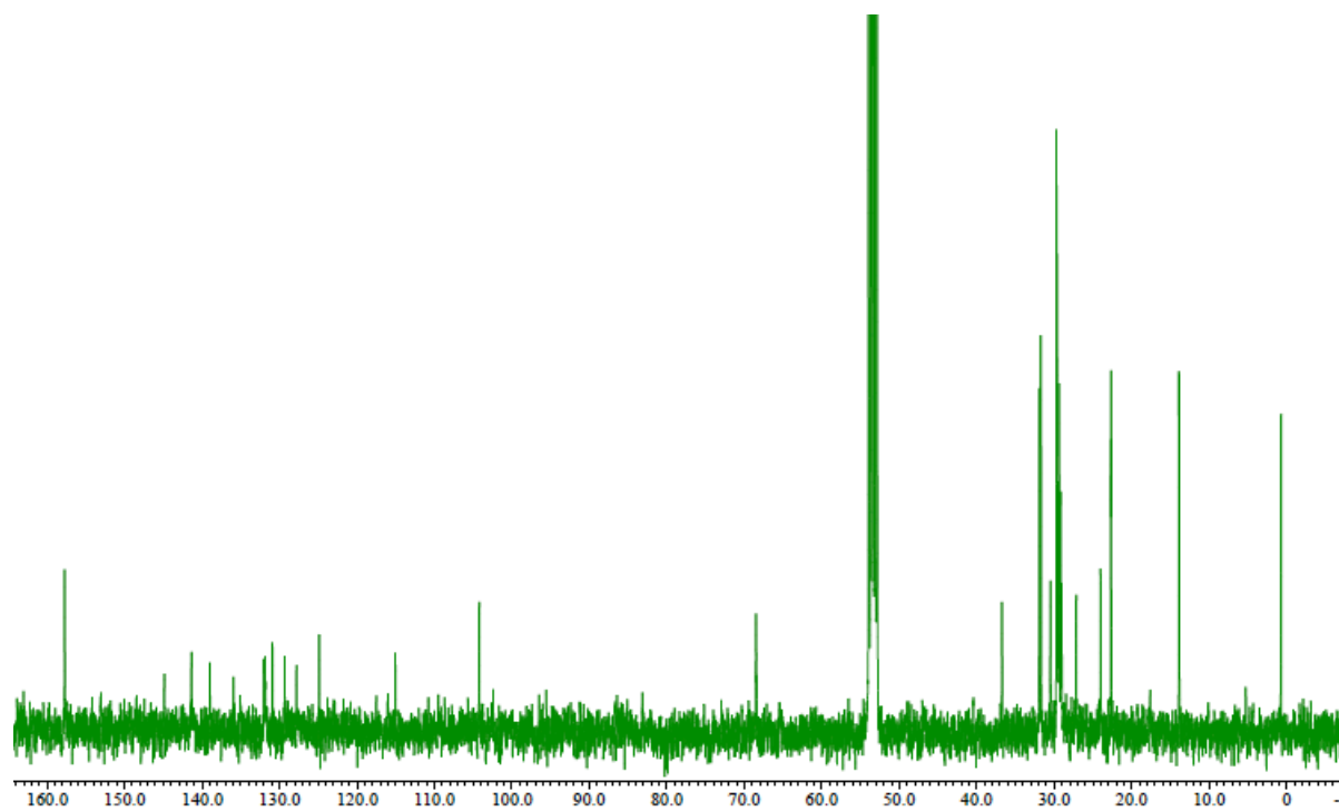
^{13}\text{C} NMR spectrum of A1
