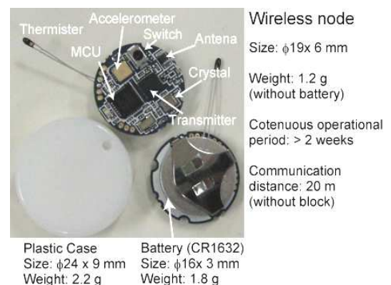
Fig. 1. Photograph of the developed prototype wireless sensor node.
