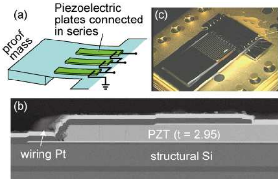
Fig. 9 (a) Schematic image of the accelerometer. (b) Cross-sectional SEM image. (c) The overview.
