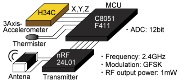
Fig. 2. Block diagram of the developed prototype wireless sensor node.
