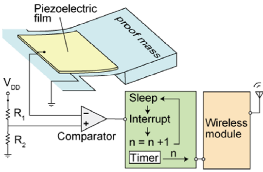
Fig. 7 Images for the concept of proposed node
