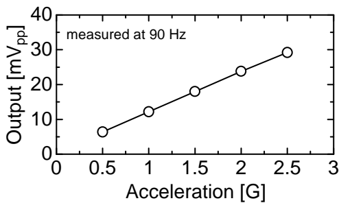
Fig. 10 Relationship between the peak-to-peak values of the output voltage for 10 PZT plates connected in series and acceleration.
