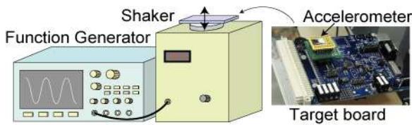
Fig. 11 Experimental setup for the investigation of the availability of comparator with hysteresis
