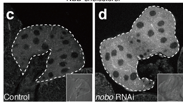
Figure 4 | Feeding rescue experiments and abnormal cholesterol accumulation in nobo loss-of-function animals. (a) Feeding rescue experiments for nobo RNAi larvae. nobo RNAi and control larvae were fed yeast paste supplemented with ethanol (EtOH, for negative control), cholesterol (C), 7-dehydrocholesterol (7dC) or 20E throughout their larval development. The concentration of each supplemented sterol in yeast paste was 0.5%(w/w) (See Methods for more details). The percentage of living animals at 240 hours AEL in each experimental condition was scored. N > 30 for each experiments. Inset photo shows nobo RNAi animals at 240 hours AEL, which were raised on food with EtOH- (right) and 20E-supplemented (left) food, respectively. The larva (right) was at the 2nd instar stage. (b) Sterol amounts in the RG isolated from control and nobo RNAi larvae. C, cholesterol; βsito, β-sitosterol; Ergo, ergosterol; Campe, campesterol. 7dC amounts were under the detectable level in our experimental conditions, and thus, the 7dC data were not included in this graph. N = 10 for each genotype. *, P < 0.05 with Student's t -test. n.s., not significant. Note that the higher level of β-sitosterol was observed in nobo RNAi PG cells, but the difference was not statistically significant. (c,d) Fluorescence and bright-field (inset) images of the PG from (c) control and (d) nobo RNAi animals incubated with 22-NBD-cholesterol. White dotted lines indicate the PG area. Scale bar: 50 μm.
