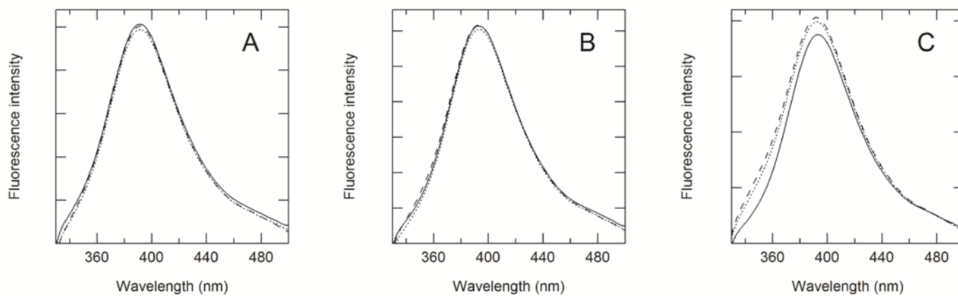
Figure S1. Fluorescence spectra of 3 \mu\text{M} methyl gallate ( C1 ) (A), ethyl gallate ( C2 ) (B) and propyl gallate ( C3 ) (C) in the presence or absence of 10 \mu\text{M} DOPC or DOPG: no lipid, solid line; DOPC, broken line; DOPG, dotted line. The excitation wavelength of the fluorescence spectra is 271 nm.
