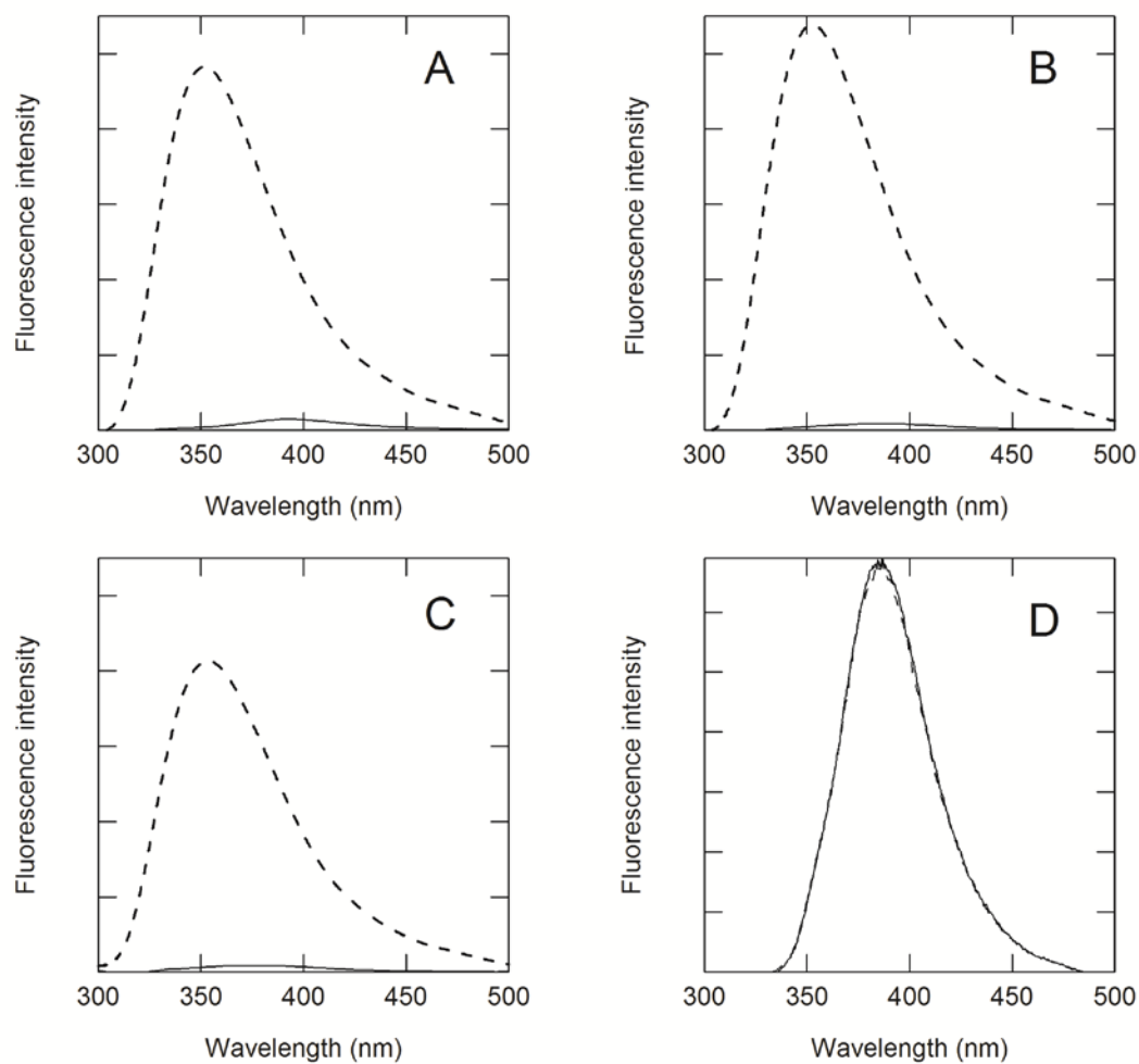
Figure S2. Fluorescence spectra of 3 \mu\text{M} octyl gallate ( C8 ) (A), dodecyl gallate ( C12 ) (B), cetyl gallate ( C16 ) (C), and stearyl gallate ( C18 ) (D) in the absence (solid lines) and presence (broken lines) of 10 \mu\text{M} DOPC. The excitation wavelength of the fluorescence spectra is 271 nm.
