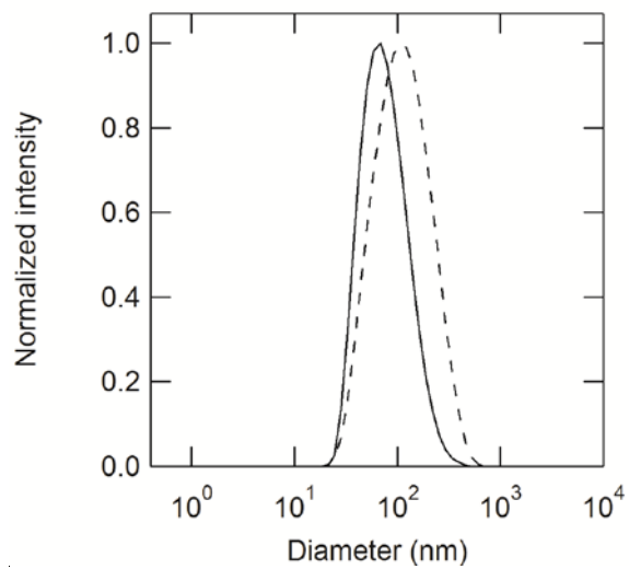
Figure 1. DLS measurements for 3 \mu\text{M} cetyl gallate ( C16 ) (solid line) and stearyl gallate ( C18 ) (broken line) in water.
