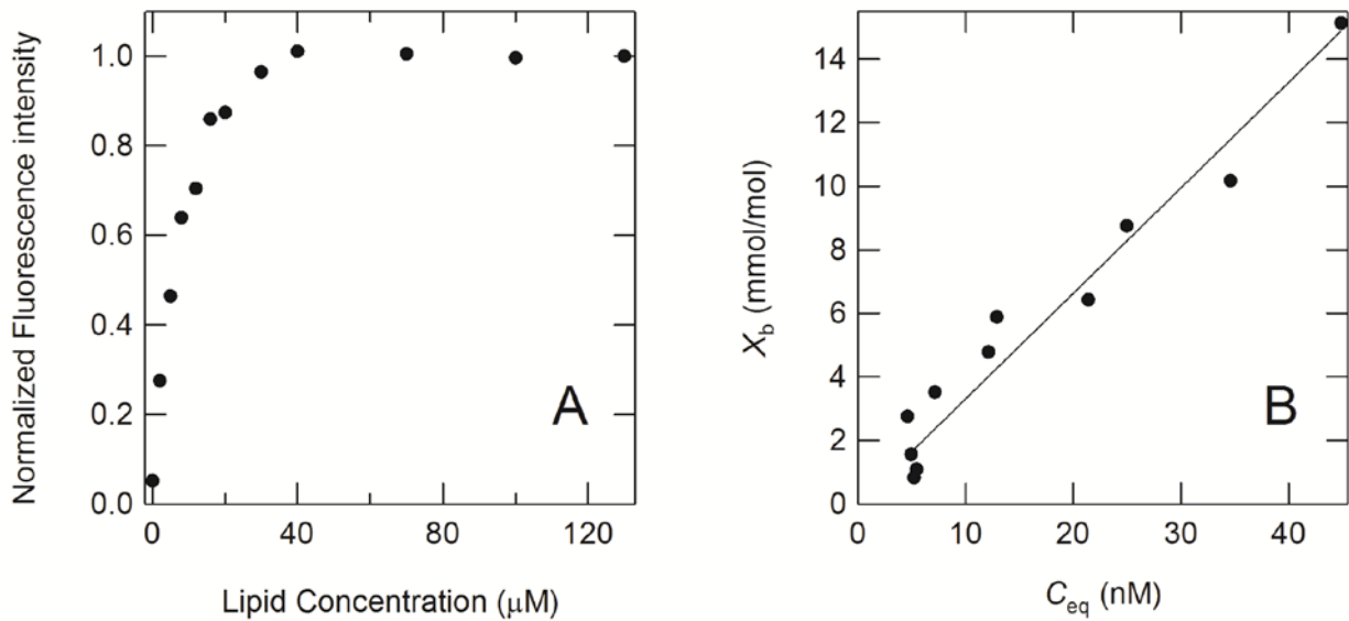
Figure 4. (A) Normalized fluorescent intensity of 60 nM octyl gallate ( C8 ) at 350 nm in various concentrations of DOPC, normalized by the maximum value. (B) Binding isotherms of octyl gallate ( C8 ) to the lipid membrane of DOPC at 25 °C.
