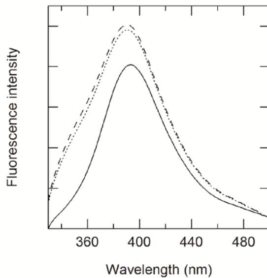
Figure 2. Fluorescence spectra of 3 \mu\text{M} butyl gallate ( C4 ) in the presence and absence of 10 \mu\text{M} DOPC or DOPG: no lipid, solid line; DOPC, broken line; DOPG, dotted line. The excitation wavelength of the fluorescence spectra is 271 nm.
