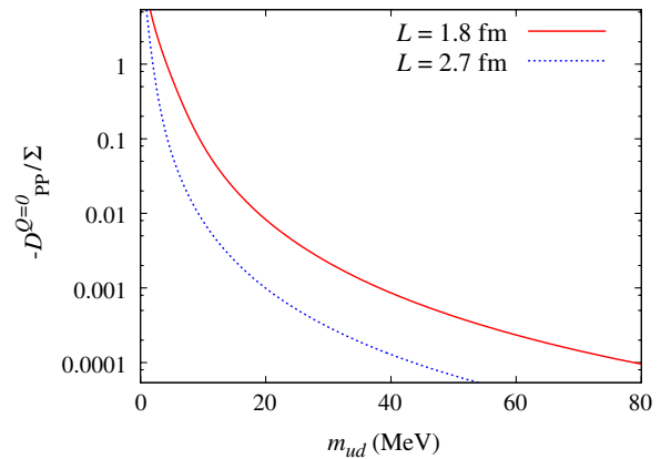
FIG. 2 (color online). The quark mass m_{ud}(=m_v) dependence of -D_{\text{PP}}^Q (normalized by \Sigma ) at Q = 0 . The same inputs as Fig. 1 are used.
