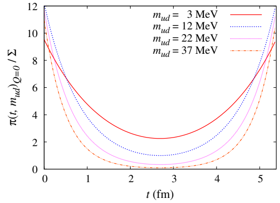
FIG. 1 (color online). The N_f = 2 + 1 ChPT prediction for the pion correlator \pi(t, m_v)_Q (normalized by \Sigma ) at Q = 0 and m_v = m_{ud} . The finite periodic box size is V = L^3 T = (1.8 \text{ fm})^3 \times (5.4 \text{ fm}) . We use m_s = 111 MeV, \Sigma^{\overline{\text{MS}}}(2 \text{ GeV}) = [234 \text{ MeV}]^3 , F = 71 MeV, L_4^r(770 \text{ MeV}) = 0.0 , L_5^r(770 \text{ MeV}) = 2.2 \times 10^{-3} , L_6^r(770 \text{ MeV}) = 0.0 and L_8^r(770 \text{ MeV}) = 1.1 \times 10^{-3} as the inputs.
