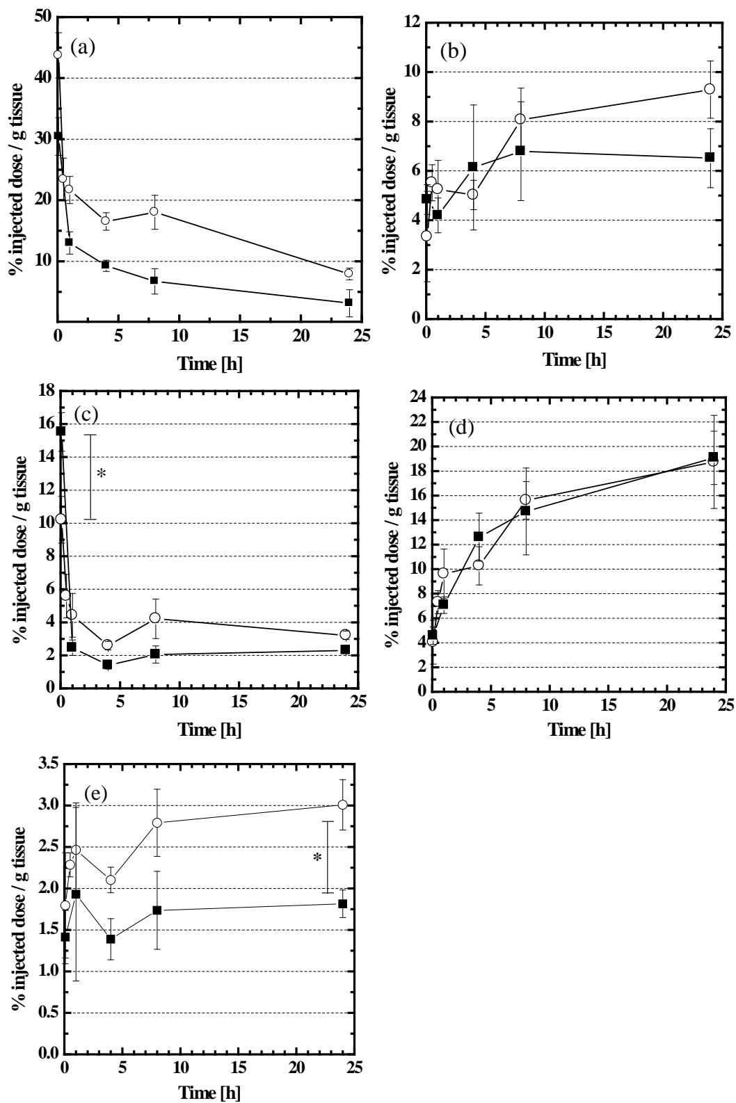
Fig. 7. Tissue distribution profiles of ^{125}\text{I} -labeled Tyr-CL micelles (open circles) and ^{125}\text{I} -labeled Tyr-NCL micelles (closed squares) in the blood (a), liver (b), kidney (c), spleen
