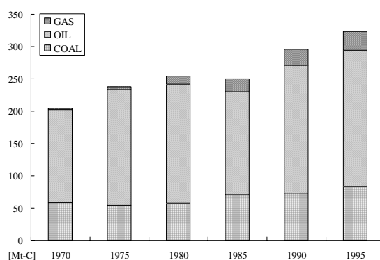
Figure 3. CO 2 emission in Japan, 1970-95
