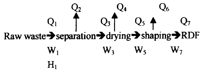
Figure 3: Basic Process for RDF Production
