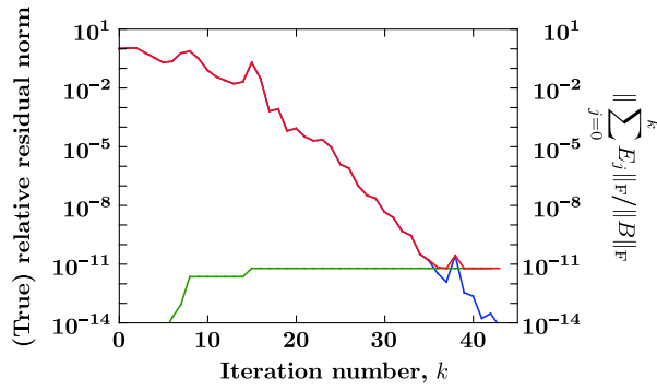
Figure 3: Relation between the true relative residual norm of Block BiCGSTAB and \|\sum_{j=0}^k E_j\|_F/\|B\|_F (JPWH991, L = 4 ). — : true relative residual norm \|B - AX_k\|_F/\|B\|_F , — : relative residual norm \|R_k\|_F/\|B\|_F , — : \|\sum_{j=0}^k E_j\|_F/\|B\|_F .
