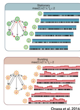
図2 Multivariate Hawkes過程と Cascading Condition
