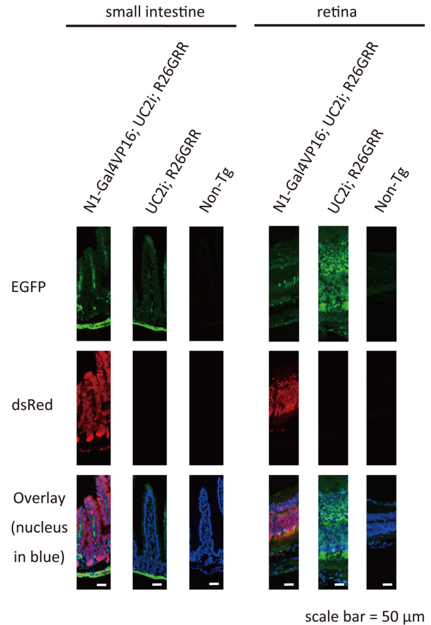
Fig. 3. Green to Red conversion after Gal4-dependent Cre recombination. Fluorescence imaging of adult intestinal epithelial cells (left panels) and retina cells (right panels). Because the cryptic stem cells of the small intestine receive Notch signaling, the intestinal epithelial cells of N1-Gal4VP16; UC2i; R26GRR mice expressed dsRed, which was absent in the UC2i; R26GRR mice and non-transgenic mice (negative controls). In addition, the retina cells of N1-Gal4VP16; UC2i; R26GRR mice expressed dsRed, which was absent in the UC2i; R26GRR mice and non-transgenic mice (negative controls).
