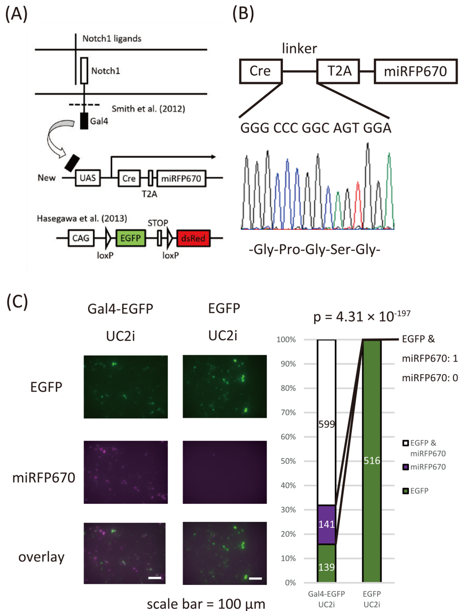
Fig. 1. Generation of UAS-Cre-T2A-miRFP670 (UC2i) mouse line. (A) Schematic representation of the reporter system. Trans-interaction of Delta ligands and Notch1-Gal4VP16 fusion protein induces translocation of Gal4VP16 to the nucleus and expression of Cre recombinase, which converts the signal from EGFP to dsRed, also triggering expression of miRFP670. Therefore, dsRed and miRFP670 signals represent past and ongoing Notch1 activity, respectively. (B) The result of direct DNA sequencing of the linker elements of UAS-Cre-T2A-miRFP670 plasmid. Note that a -Gly-Ser-Gly- coding sequence is present at the N terminus of T2A sequence. (C) In vitro examination for Gal4 dependency of the expression of miRFP670. 293T cells were transfected with the indicated expression vectors and photographed with the GFP or Cy5 filter. The cumulative bar graph showed the result of statistics of the transfected cells.
