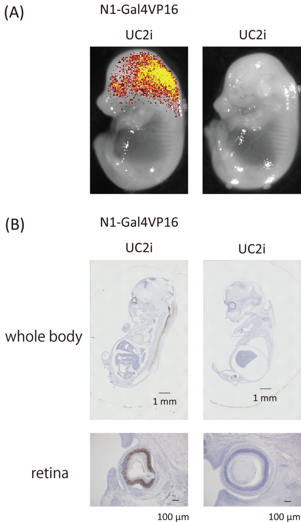
Fig. 2. Whole body imaging of miRFP670 fluorescence imaging signal. (A) The eye and a part of the head region of N1-Gal4VP16; UC2i embryos (E14.5) showed strong miRFP670 signals in the eye, whereas that of UC2i embryos showed no signals. (B) Immunohistochemistry for Cre recombinase. Note that the neural cells of the retina of N1-Gal4VP16; UC2i embryos were positive for Cre recombinase.
