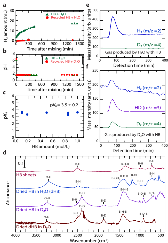
Fig. 2 Proton exchange reaction and hydrolysis reaction of HB and recycled HB sheets in water. a H 2 amount as a function of time for the mixture of H 2 O (2.0 mL) and HB sheets (100 mg) and that for the recycled HB (HB dried at 353 K after 1440 min from the mixture with H 2 O). b pH change as a function of time for the mixture of H 2 O (2.0 mL) and HB sheets (100 mg) and that for D 2 O and the recycled HB (HB dried at 353 K after 1440 min from the mixture with H 2 O). c pK a derived from the pH change after mixing water and HB sheets with various HB amount. d Fourier transform infrared absorption spectroscopy results for the HB sheets, the recycled HB sheets obtained by drying the mixture of HB and H 2 O after 1440 min after mixing (dHB), recycled HB obtained by drying HB in D 2 O after 1440 min after mixing, and recycled dHB obtained by drying the mixture of dHB and D 2 O after 1440 min after mixing. The assignment of the absorption peaks was based on the previous report 21 . e Mass analysis of produced gas after the mixing H 2 O and HB sheets. m/z denotes the mass-to-charge ratio. f Mass analysis of produced gas after the mixture of D 2 O and HB sheets. The horizontal axis in (e) and (f) indicates time after injection of produced gas in the apparatus.
