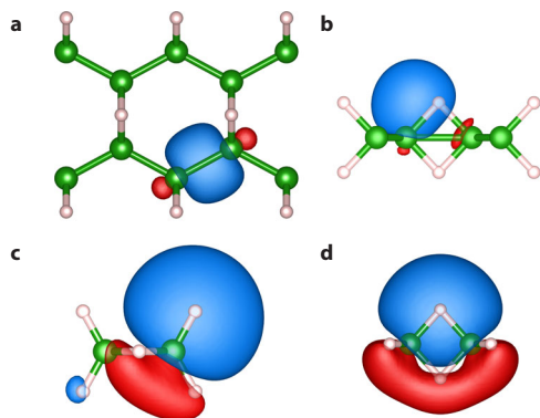
Fig. 7 MLWFs on the HB sheet. The isosurfaces of the MLWFs on the HB sheet ( a, b ) and B_2H_6 ( c, d ) are shown. Only the inequivalent MLWFs are shown. Blue (red) surfaces indicate positive (negative) isovalue.
