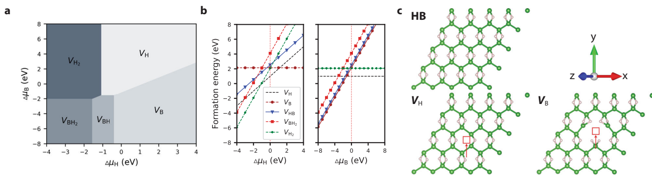
Fig. 4 Formation of vacancy-defective HB sheet. a Phase diagram for the stable defect in HB in the (\Delta\mu_{\text{H}}, \Delta\mu_{\text{B}}) space. b Formation energy as a function of \Delta\mu_{\text{H}} at \Delta\mu_{\text{B}} = 0 (left) and that as a function of \Delta\mu_{\text{B}} at \Delta\mu_{\text{H}} = 0 (right). c Visual representation of the optimized structures of pristine, H vacant ( V_{\text{H}} ) and B vacant ( V_{\text{B}} ) HB sheets. Positions of H and B atoms removed are indicated by open squares.
