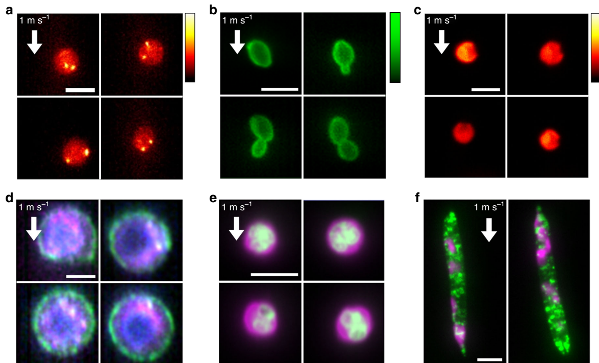
Fig. 3 Fluorescence images of diverse cell types obtained by VIFFI flow cytometry. All the images were obtained at a flow speed of 1 m s -1 . a FISH images of Jurkat cells. Two bright spots (shown in yellow-white) corresponding to two copies of chromosome 8 are evident in each cell. b Fluorescence images of S. cerevisiae whose cell wall was stained by FITC-concanavalin A, showing budding daughter cells from their mother cells. c Autofluorescence images of C. reinhardtii cells, showing their characteristic morphological features (indented elliptical shape at the head). d Three-color fluorescence images of human lung adenocarcinoma cells (PC-9). Magenta: protoporphyrin IX induced by 5-aminolevulinic acid; Green: EpCAM stained by VU-1D9; Blue: nucleus stained by Hoechst 33342. e Two-color fluorescence images of murine neutrophils. Green: nucleus stained by SYTO16; Magenta: cytoplasm stained by CellTracker Red. f Two-color fluorescence images of E. gracilis cells. Green: lipids stained by BODIPY505/515; Magenta: autofluorescence of chlorophyll. Scale bars: 10 μm.
