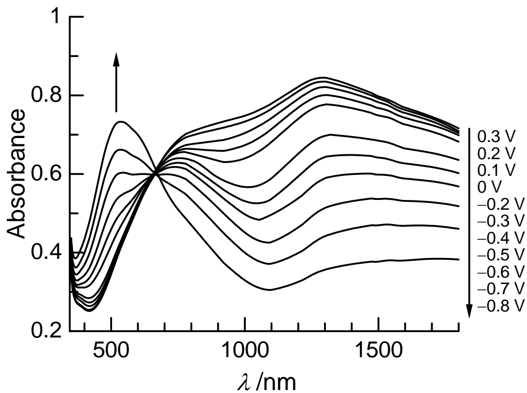
Fig. S1 Ultraviolet–visible–near-infrared absorption spectra at various potentials vs Fc/Fc +
