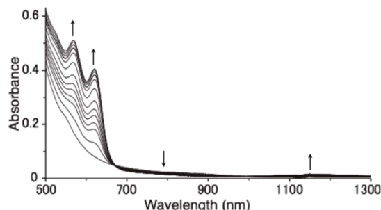
Fig.2. Visible-NIR spectra of \text{La}_2@\text{C}_{80} ( 1.0 \times 10^{-4} M) in the presence of TMPD (0-10 equiv).
