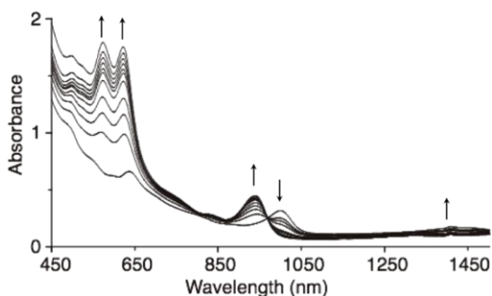
Fig.1. Visible-NIR spectra of \text{La}@\text{C}_{82} ( 1.0 \times 10^{-4} M) in the presence of TMPD (0-10 equiv).
